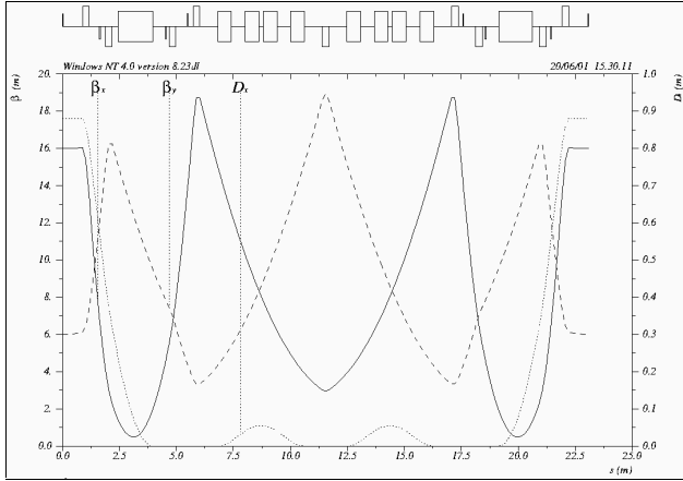
Figure 2: Lattice functions in the chicane section.
