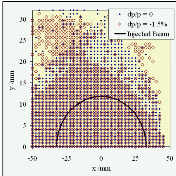
Figure 5: Dynamic aperture for on-momentum particles, and particles with -1.5\% momentum deviation.
