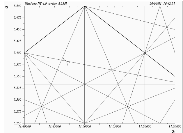
Figure 4: Working point of the lattice in tune space.
