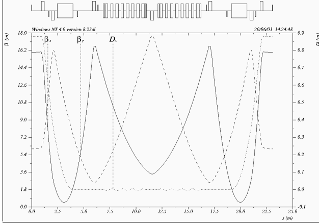
Figure 1: Lattice functions in the wiggler section.
