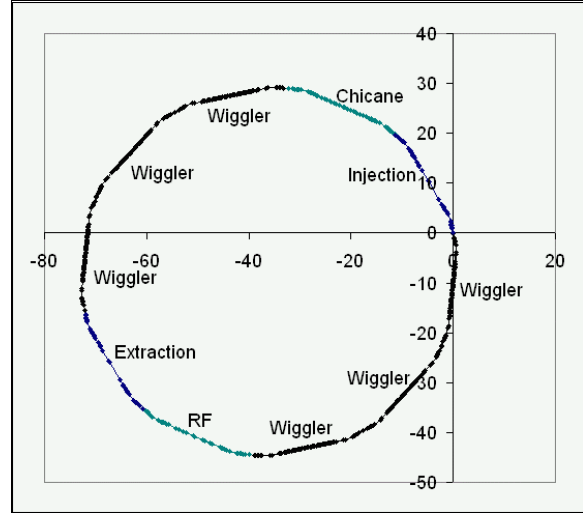
Figure 3: Pre-damping ring structure. Horizontal and vertical scales are in metres.
