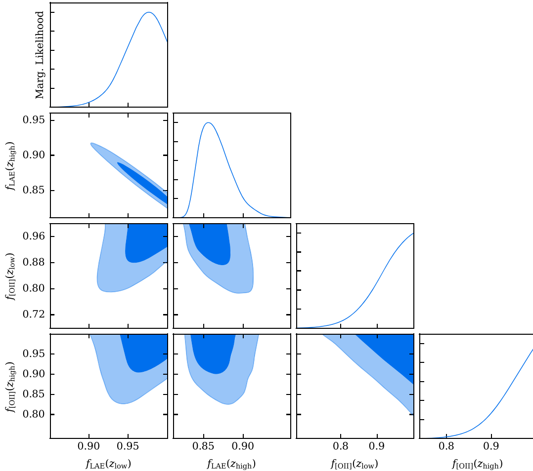
Figure 8. The 68 and 95 per cent MCMC contours derived by fitting the cross-correlation function of the mock catalogues using a two parameter model for the purity to the LAE and [O II] samples. These results are from our lightcone decontamination method. The data are for the high-contamination P_{\text{LAE}} > 0.15 sample, which has an average contamination rate of 7 per cent. The normalized, marginalized 1D likelihoods are also shown. A redshift dependence of the contamination of the LAEs is clearly detected.
