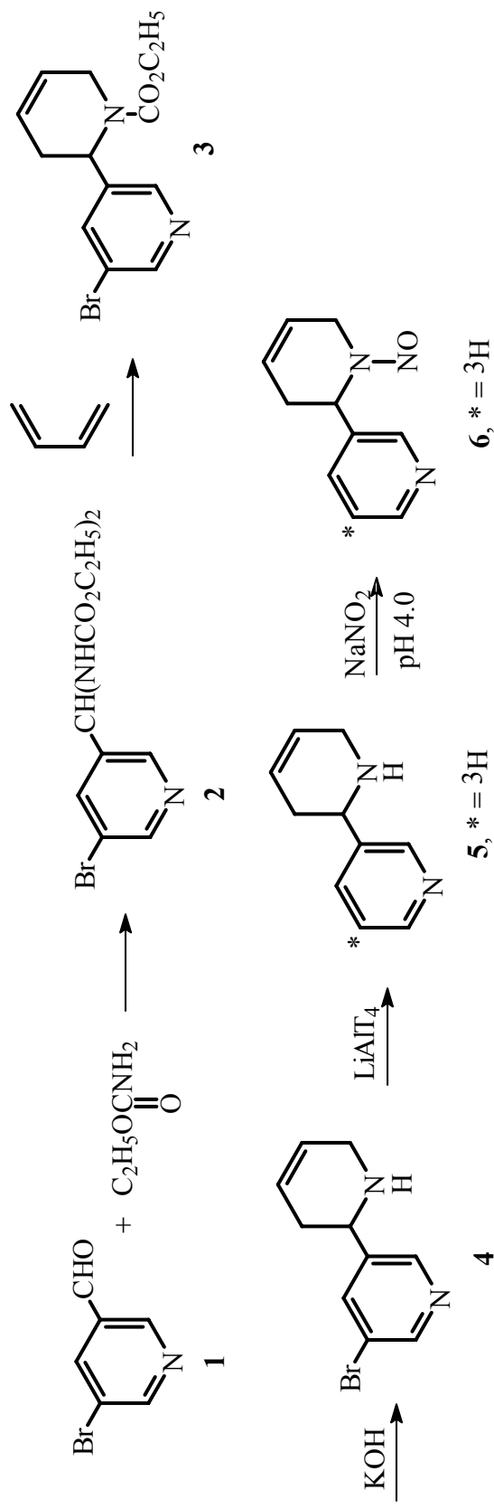
Scheme I: Synthesis of [5-3H]nitrosoanatabine (6)
