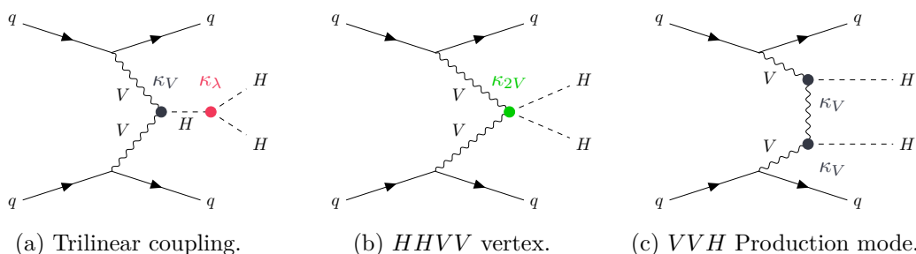
Figure 2. The VBF production of Higgs boson pairs via (a) the trilinear coupling, (b) the HHV V vertex, and (c) the V V H production mode. In the figure, \kappa_V and \kappa_{2V} denote the HV V and HHV V coupling strength modifiers.
