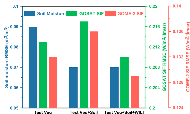
Figure 6. Global root-mean-square error (RMSE) of different experiments relative to Soil Moisture and Ocean Salinity (SMOS) soil moisture and Greenhouse gases Observing SATellite (GOSAT) and Global Ozone Monitoring Experiment-2 (GOME-2) solar-induced chlorophyll fluorescence (SIF).
