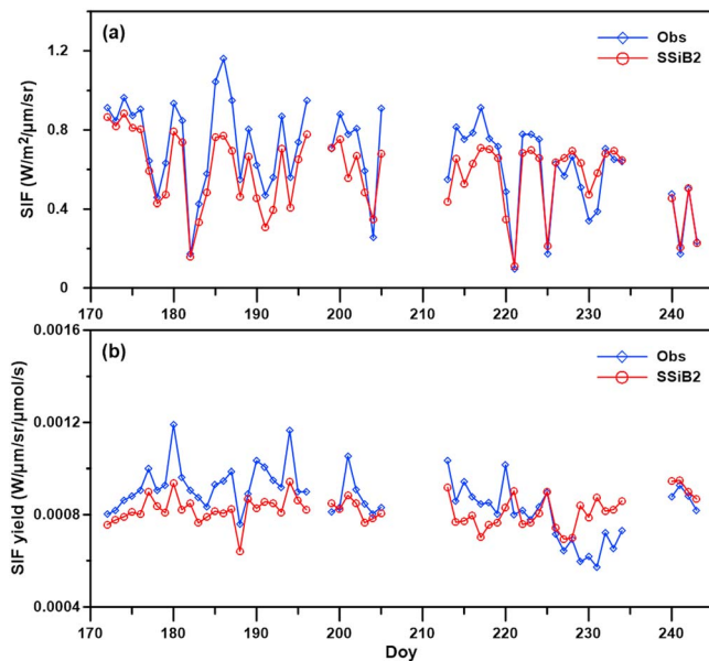
Figure 1. Daily mean solar-induced chlorophyll fluorescence (SIF) and SIF yield over the flux tower site at Harvard Forest, USA (42.538°N, 72.171°W). Blue line represents measured values over the flux tower, and red line represents the Simplified Simple Biosphere Model version 2.0 (SSiB2) result.
