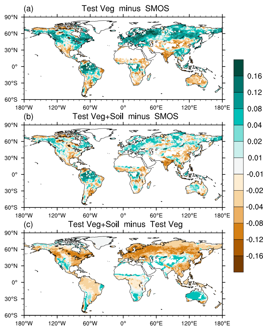
Figure 5. Global difference of soil moisture, units: \text{m}^3/\text{m}^3 . (a) Test Veg – Soil Moisture and Ocean Salinity (SMOS), (b) Test Veg+Soil – SMOS, (c) Test Veg+Soil – Test Veg.
