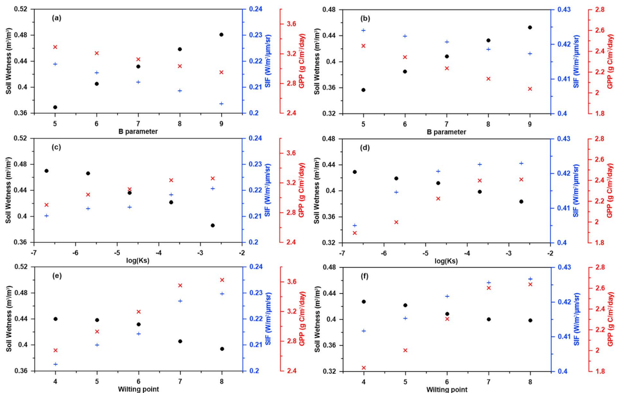
Figure 10. Calculated soil moisture (black), solar-induced chlorophyll fluorescence (SIF) (blue), and gross primary production (GPP) (red) for savanna (a, c, and e) and grassland (b, d, and f), (a and b) B parameter; (c and d) logarithm of K_s ; (e and f) wilting point.
