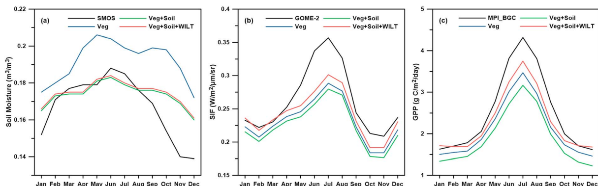
Figure 9. The monthly mean (a) soil moisture, (b) solar-induced chlorophyll fluorescence, and (c) gross primary production at the global scale in Test Veg, Test Veg+Soil, and Test Veg+Soil+WILT. SMOS = Soil Moisture and Ocean Salinity.
