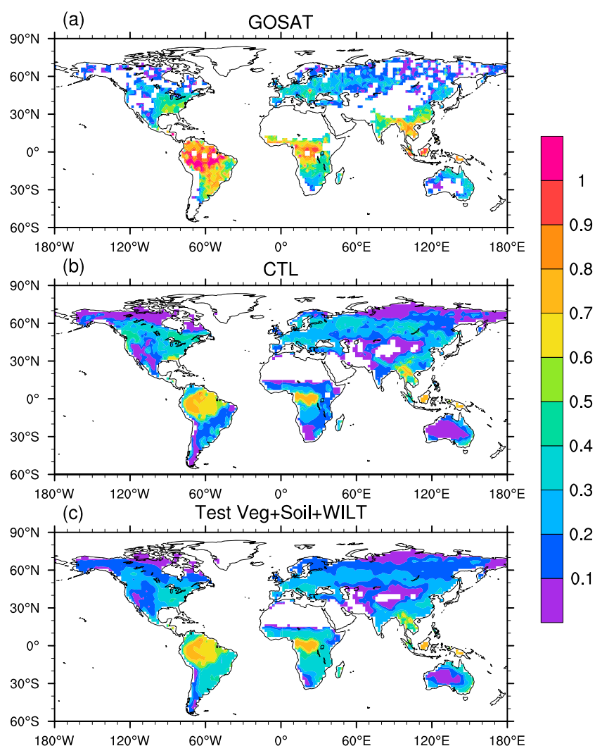
Figure 3. Global map of annual mean solar-induced chlorophyll fluorescence (SIF) from 2009 to 2012, units: \text{W/m}^2/\mu\text{m}/\text{sr} . (a) Greenhouse gases Observing SATellite (GOSAT), (b) control run (CTL), and (c) Test Veg+Soil+WILT.
