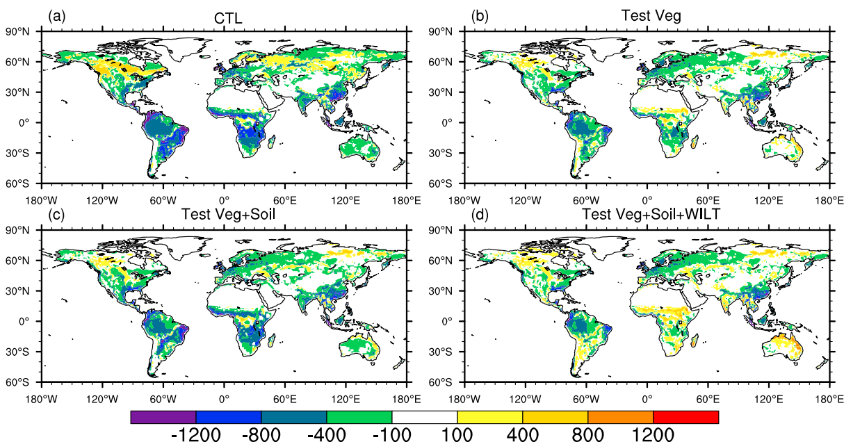
Figure 7. Global difference of gross primary production between MPI-BGC and the experiments, units: \text{g C}/\text{m}^2/\text{yr} . (a) Control run (CTL), (b) Test Veg, (c) Test Veg+Soil, (d) Test Veg+Soil+WILT.
