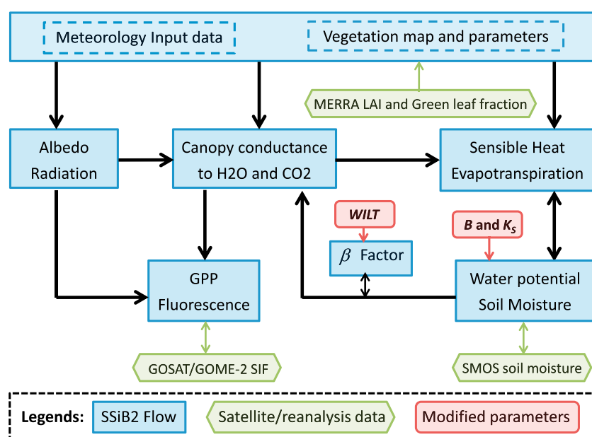
Figure 2. Overview flowchart of the Simplified Simple Biosphere Model version 2.0 (SSiB2) land surface model and the modified parameters in the model. The blue boxes are the SSiB2 flowchart; the green boxes are the satellite/reanalysis data; and the red boxes are the modified parameters in the model. GPP = gross primary production; MERRA = Modern-Era Retrospective Analysis for Research and Applications; LAI = leaf area index; GOSAT = Greenhouse gases Observing SATellite; GOME-2 = Global Ozone Monitoring Experiment-2; SMOS = Soil Moisture and Ocean Salinity.
