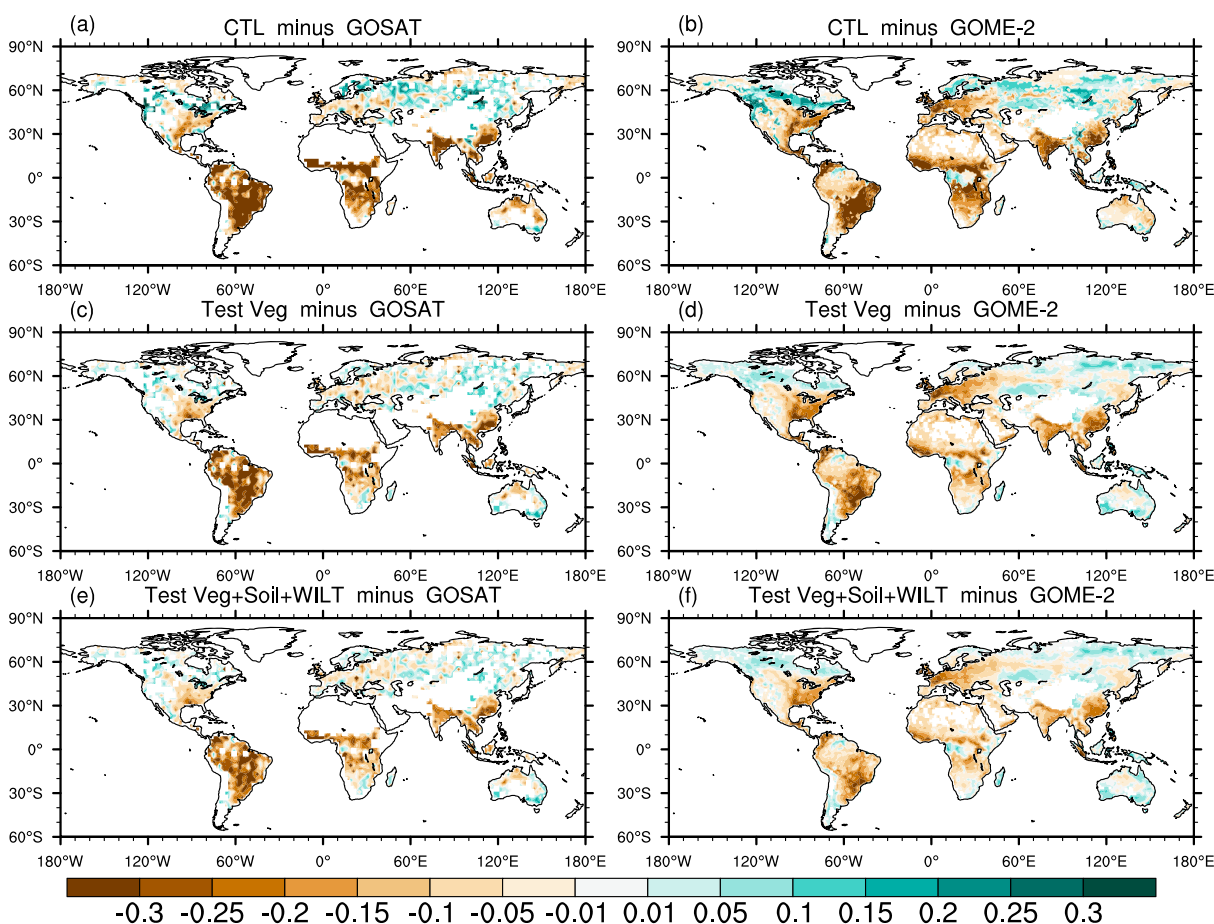
Figure 4. Global differences of annual mean solar-induced chlorophyll fluorescence compared to Greenhouse gases Observing SATellite (GOSAT) and Global Ozone Monitoring Experiment-2 (GOME-2) data, units: \text{W/m}^2/\mu\text{m/sr} . (a) CTL minus GOSAT, (b) CTL minus GOME-2, (c) Test Veg minus GOSAT, (d) Test Veg minus GOME-2, (e) Test Veg+Soil+WILT minus GOSAT, and (f) Test Veg+Soil+WILT minus GOME-2.
