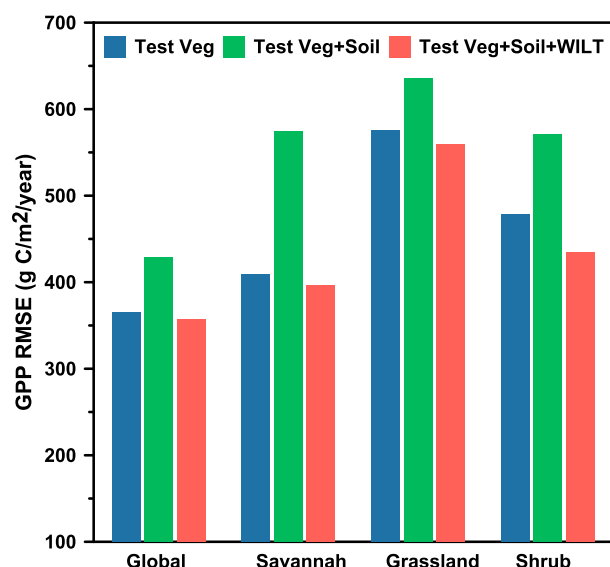
Figure 8. Root-mean-square error (RMSE) of gross primary production (GPP) from different vegetation types, units: \text{g C/m}^2/\text{yr} .
