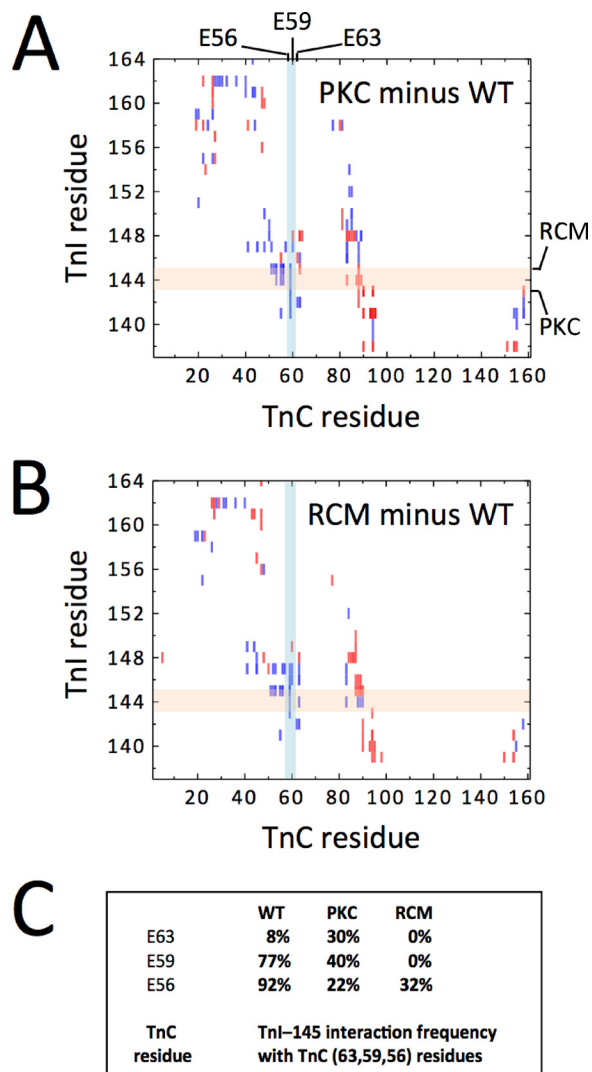
FIGURE 6. Interaction between cTnC and cTnI. Contact maps between cTnC ( abscissa ) and cTnI ( ordinate ) simulated for the PKC phosphomimetic (A) or the RCM mutant (B) were calculated from three independent production runs. In each panel, a differential map is constructed by subtracting the WT contact map and subsequently color-coded such that blue represents a decrease and red represents an increase in contact frequency. C summarizes contact frequencies between cTnI residue 145 and cTnC helix C Glu-56, Glu-59, and Glu-63 as indicated by the lightly shaded colored bars . PKC phosphomimetic significantly reduced contact between these residues, whereas the RCM R145W mutation virtually eliminated all contacts.
