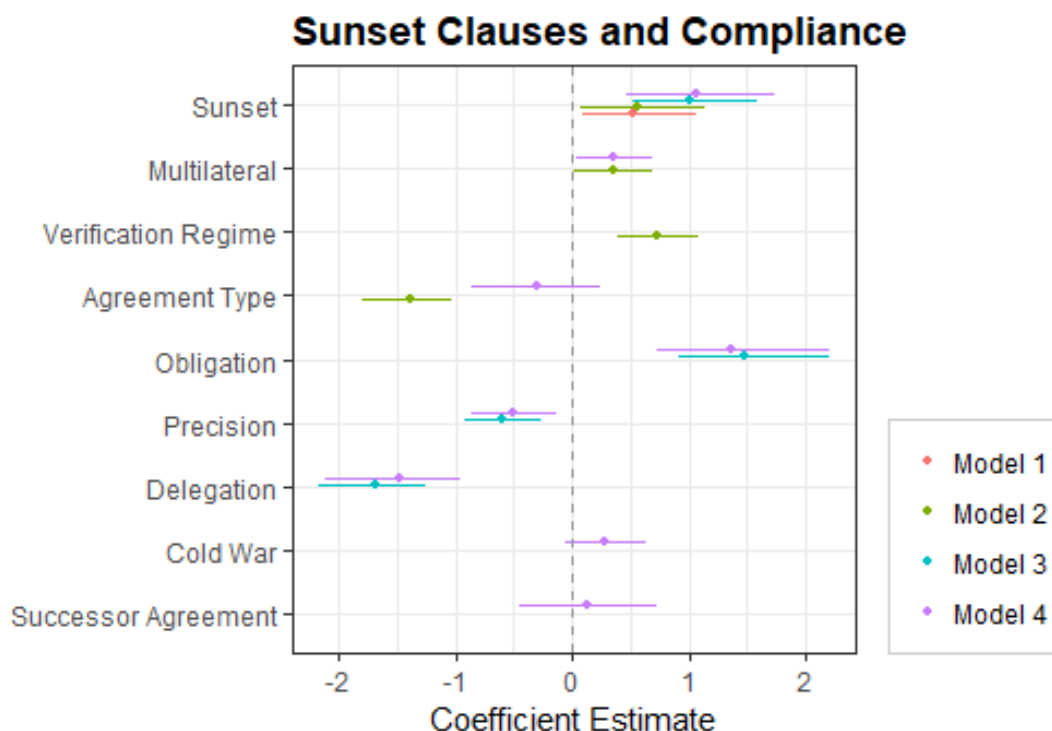
Figure 6.2: This figure graphs the results of the probit regression equation in Table 6.1.
