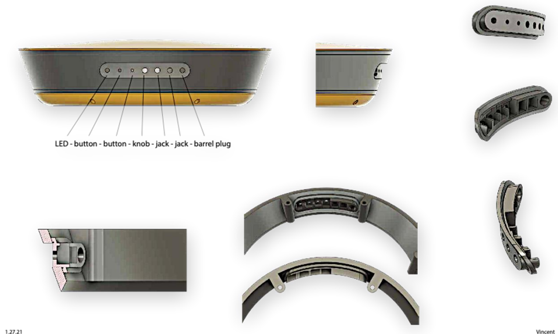
Figure 44: Renderings showing all the components that make up the RX 300 I/O schema
