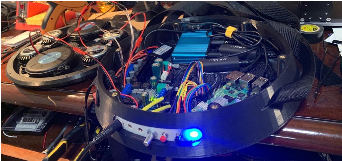
Figure 57: RX301 prototype - March 24, 2021
