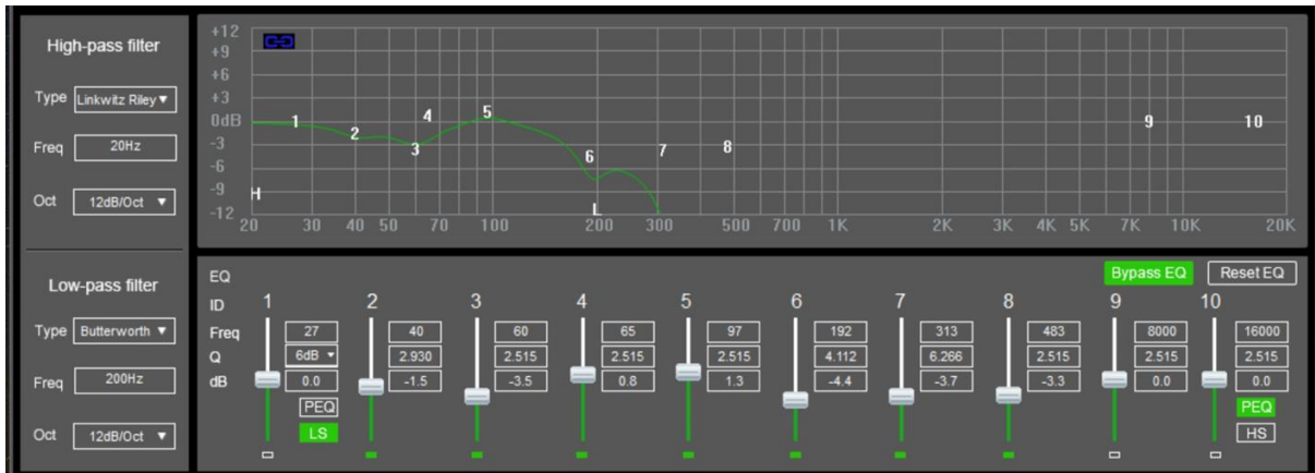
Figure 12: Low frequency settings of chair prototype
