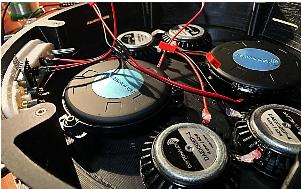
Figure 51: Transducers in RX300 RP, surrounded by the mid wall and I/O panel
