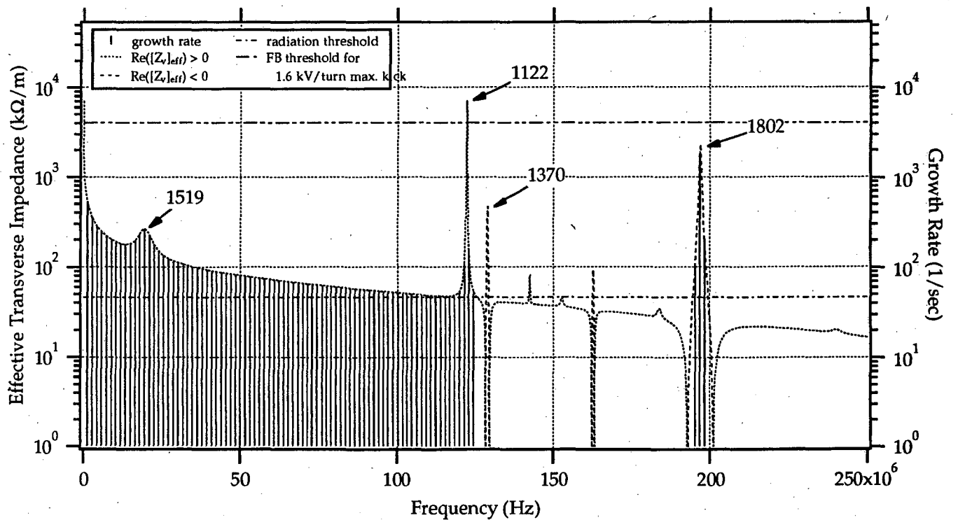
Figure 2: Vertical coupled-bunch growth rates and the effective impedance in the 0-250 MHz frequency band from the RF cavity dipole HOM and the resistive wall impedance.
