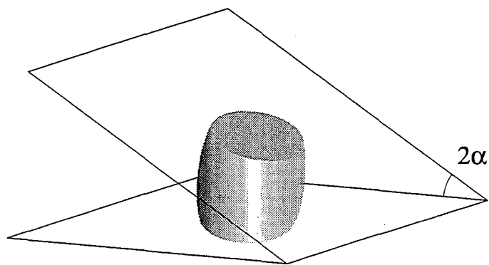
Figure 1. Tubular bridge in a wedge.
