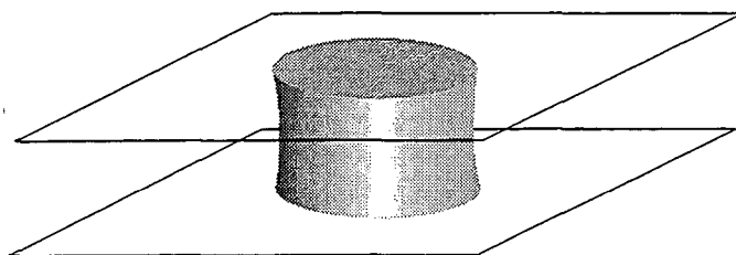
Figure 2. Bridge between parallel plates.
