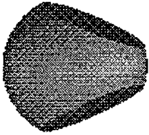
Spherical bridge \gamma - \alpha > \pi / 2
