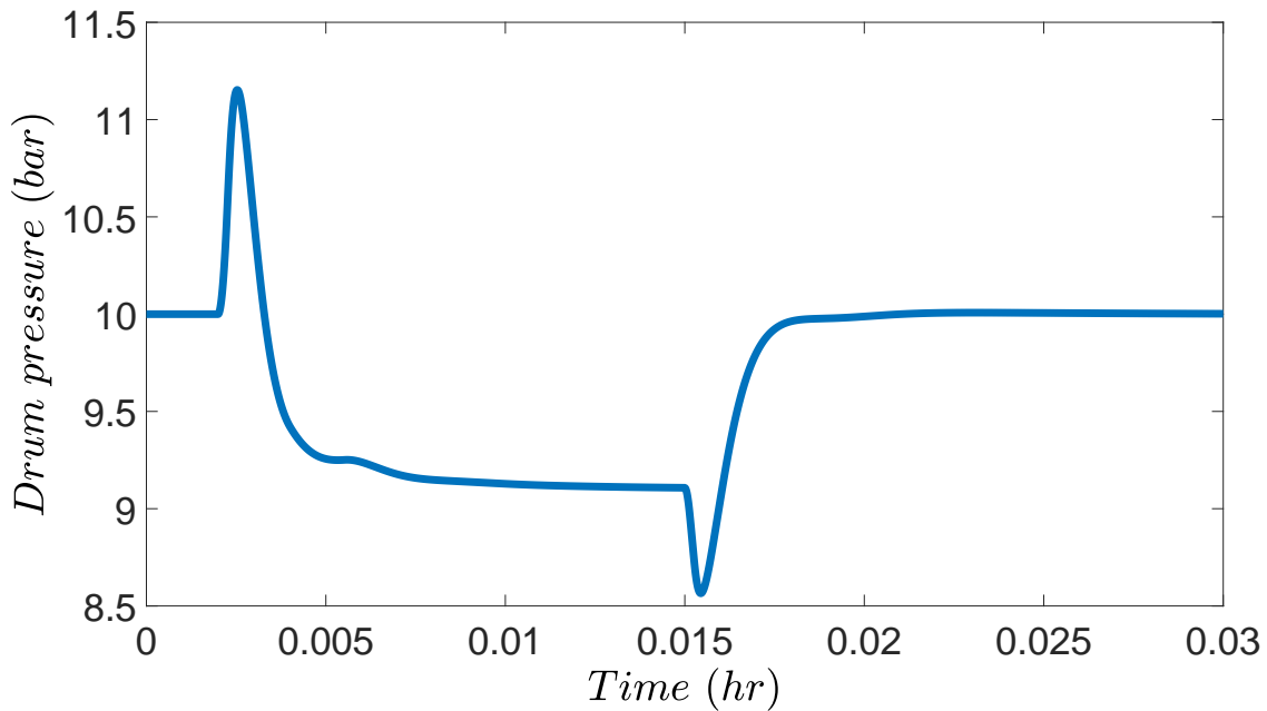
Figure 6.2: Drum pressure for the flash drum process with a varying tuning of the temperature controller to account for the activation of the safety system.
