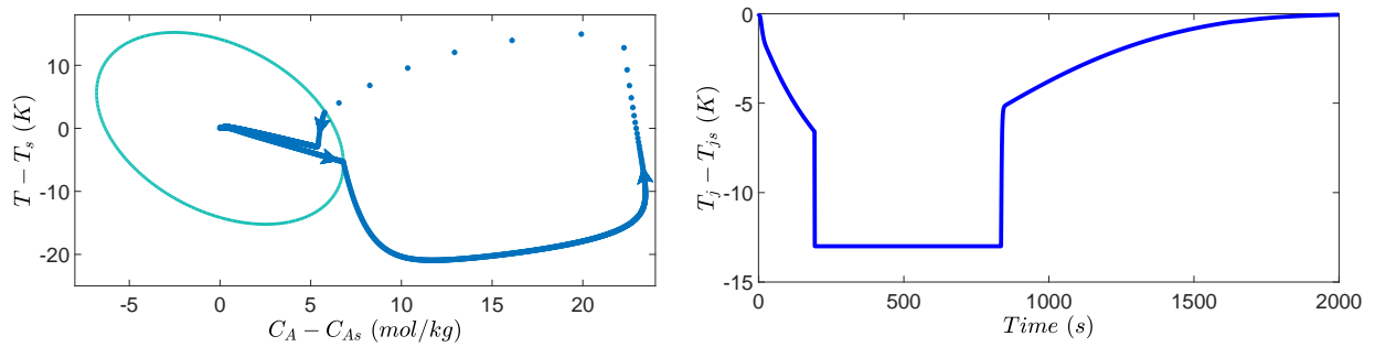
Figure 4.3: State-space plot and input plot of LMPC integrated with the safety system for the MIC hydrolysis reaction in a CSTR. The drop in the coolant temperature when the state exits the stability region is noticeable until the state re-enters the stability region and the LMPC begins to be used once again to manipulate T_j and drive the process state toward its steady-state value. The time interval is the same between the plotting of each data point in the state-space plot. Therefore, the large differences in the state between plotted points as the system approaches thermal runaway indicate rapid changes in temperature. The large differences in the state between plotted points as the state is driven back toward the stability region after the safety system is activated indicate the effectiveness of the safety system's actions to rapidly move the state back toward the stability region.
