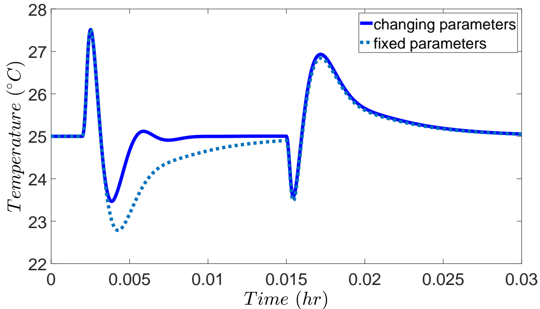
Figure 6.3: Temperature in the flash drum, with a varying tuning of the temperature controller (“changing parameters”) to account for the activation of the safety system and with no change in the tuning of the temperature controller (“fixed parameters”) when the safety system is activated.
