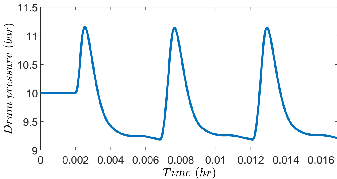
Figure 6.5: Drum pressure for the flash drum process with a varying tuning of the temperature controller to account for the activation of the safety system when the resetting pressure of the relief valve is set at 9.2 bar.
