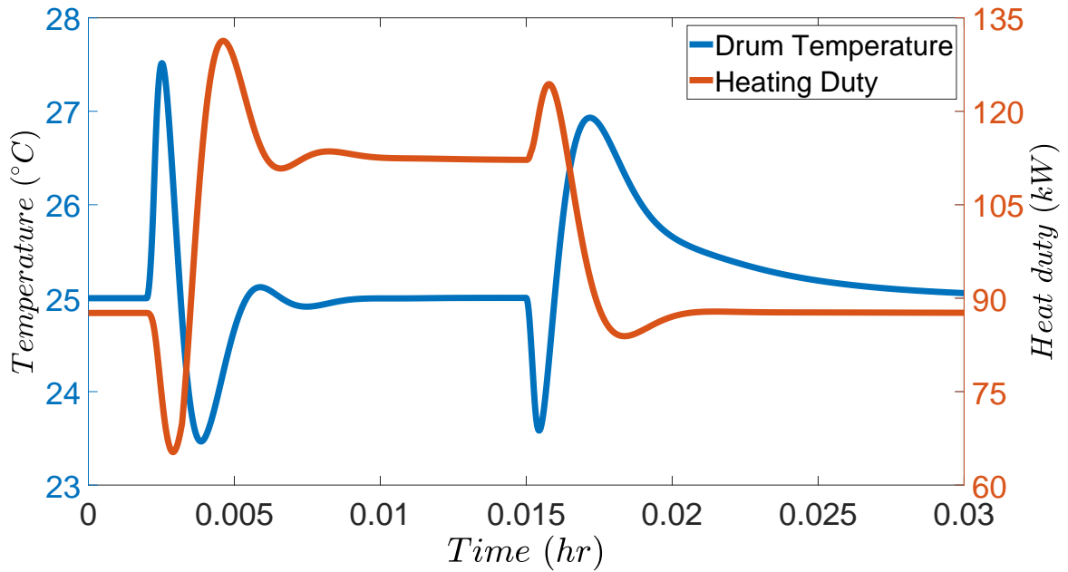
Figure 6.1: Controlled output and manipulated input for the temperature controller of the flash drum process with the tuning varying to account for the activation of the safety system.
