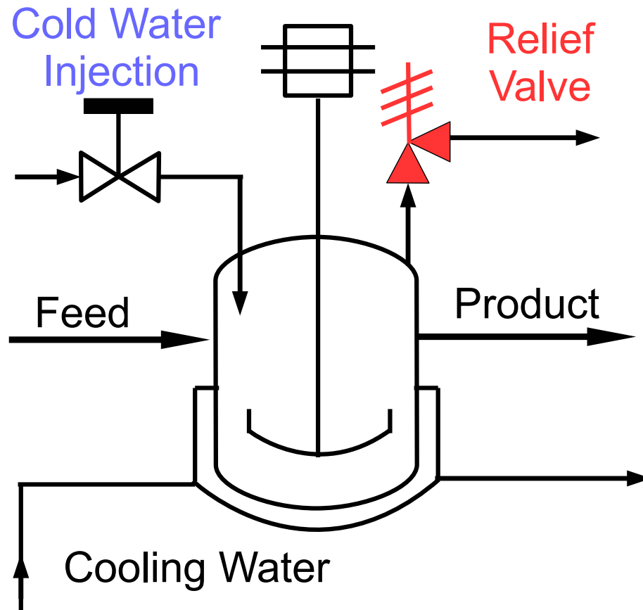
Figure 4.1: CSTR with safety system for MIC hydrolysis example. The relief valve and valve that opens to allow the cold water injection are depicted. The temperature of the cooling water is controlled by the LMPC; the positions of the two valves on the cooling water inlet and outlet for the CSTR are assumed to be fixed in this example.
