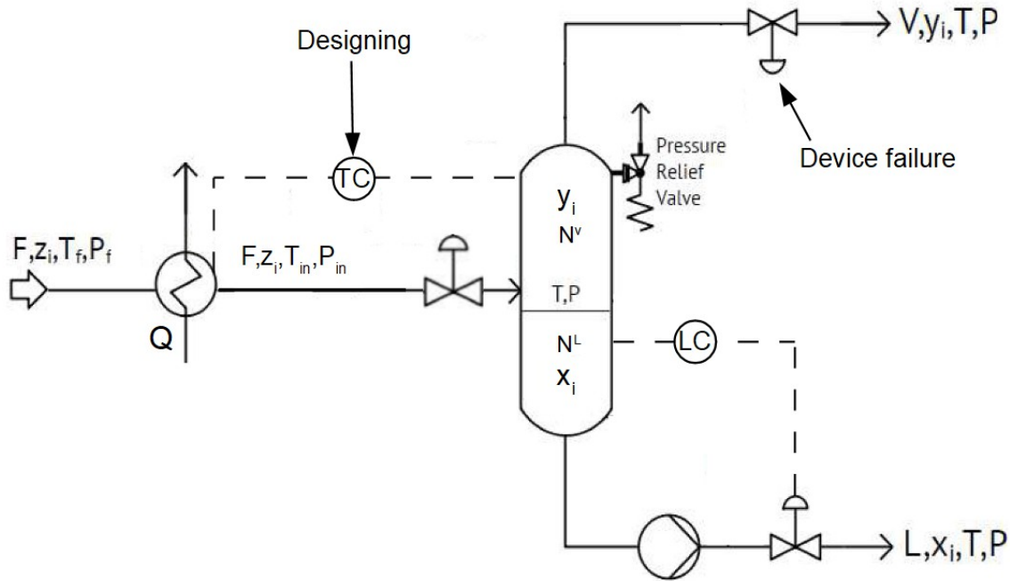
Figure 5.1: A schematic of the flash process. The temperature controller for which the tuning is changed to account for safety system activation is pointed out in the figure with the word “Designing.” The vapor effluent valve experiencing the failure is pointed out in the figure with “Device failure.” The three units shown in the figure besides the valves and controllers are, from left to right, a heat exchanger, flash drum, and pump.
