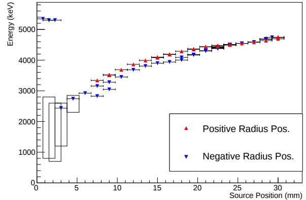
FIG. 5. The centroids of the \alpha energy peaks in each data set; certain positions were studied in multiple data sets. Negative (positive) radius positions are indicated by blue downward-pointing (red upward-pointing) triangles. For scanning positions with significant low-energy tailing, the black box depicts the estimated full energy range of \alpha events. At positions that are partially or completely incident on the point-contact, an additional peak appears at nearly the full incident \alpha energy. The vertical error bars (not visible) depict the uncertainty in the peak position from the maximum-likelihood fit of the peaks, and the horizontal errors depict the 0.75 mm estimated uncertainty of the source position.
