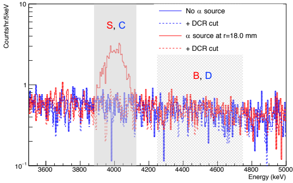
FIG. 9. The energy spectra measured with the TUBE detector without the \alpha source incident on the passivated surface, in blue, and with the source incident at r=18.0 mm, in red. Spectra are shown before (the solid lines) and after (the dashed lines) the application of the DCR cut.
