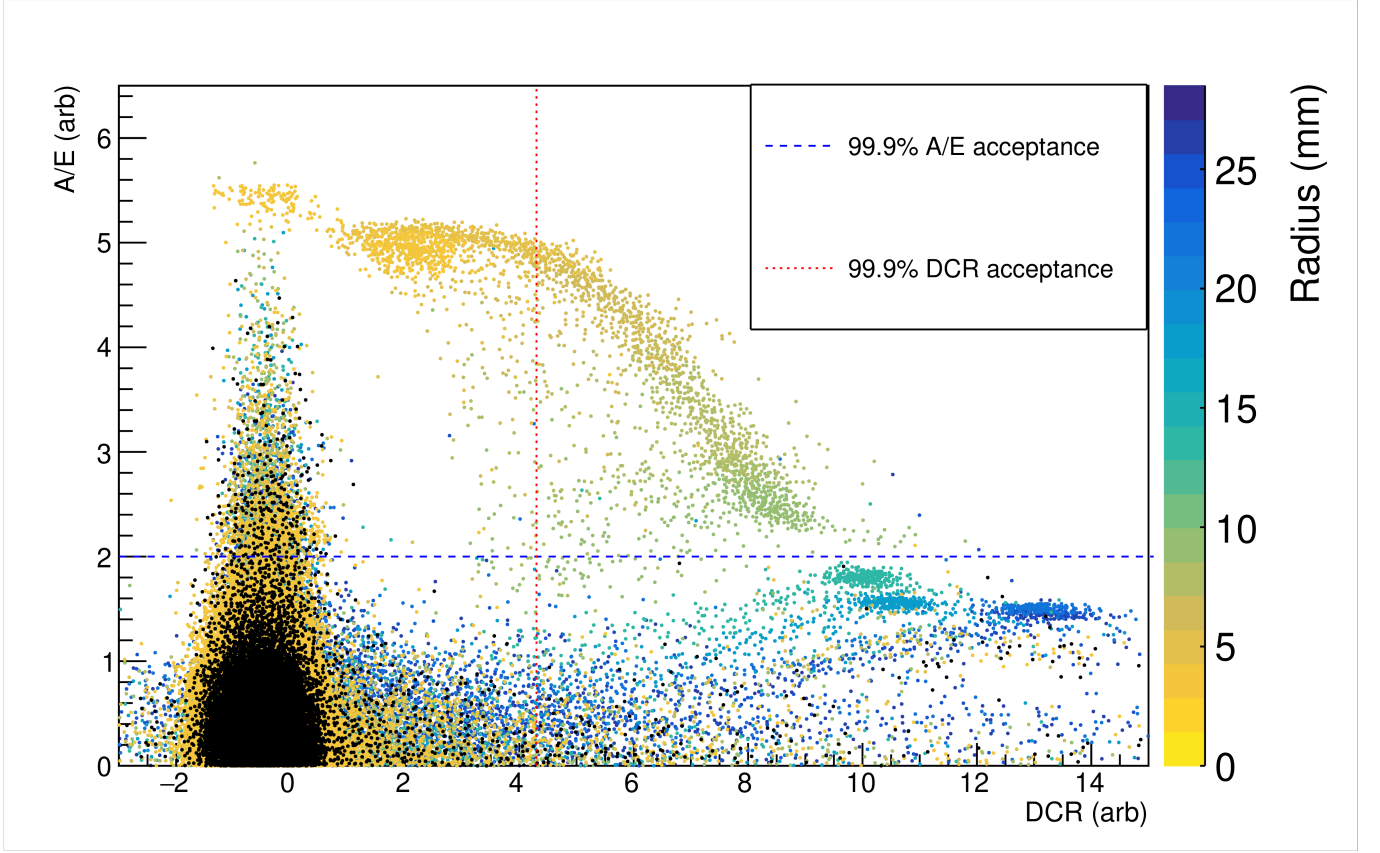
FIG. 8. The distribution of A/E and DCR values for a range of scanning positions (indicated by the color scale) and a data set with no \alpha source shining on the detector surface (in black). All single-site non-muon events with energies between 1 and 6 MeV are included. The dashed blue line indicates the 99.9% acceptance value of A/E and the dotted red line indicates the 99.9% acceptance value of DCR.
