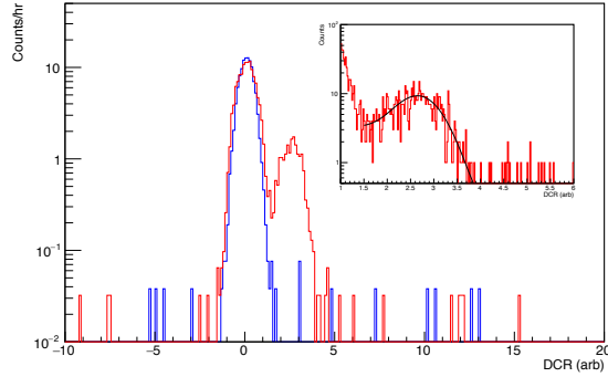
(b) The DCR distribution of single-site non-muon events with energies between 0.5 and 6 MeV and A/E > 1.5 without the \alpha source incident on the passivated surface ( in blue ), and with the source incident at r = 1.5 mm ( in red ).
