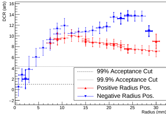
FIG. 7. The centroids of the DCR peaks in each data set; certain positions were studied in multiple data sets. Negative (positive) radius positions are indicated by blue downward-pointing (red upward-pointing) triangles. The vertical error bars give the 5\sigma -width of the DCR distribution peaks, and the horizontal errors depict the 0.75 mm estimated uncertainty of the source position. The dashed (dotted) line indicates the 99% (99.9%) bulk event acceptance DCR cut.
