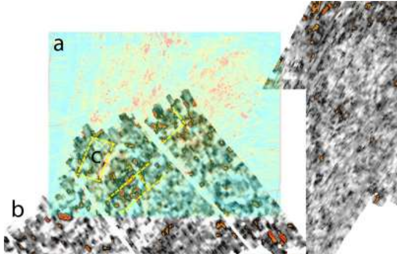
FIGURE 9 Comparison of a) top view and b) cloud to cloud target-less automatic registration of point clouds of Çatalhöyük GDA and TPC areas in FARO SCENE 5.4
