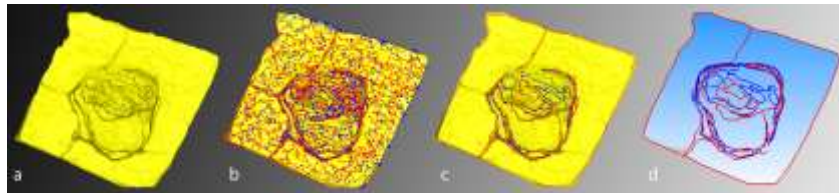
FIGURE 7 Semi-automatic feature extraction in 3D Reshaper - a) triangular mesh of Skeleton 30928 excavated in Building 89 at Çatalhöyük; b) automatic convex and concave lines detection; c) semi-automatic lines filtering; semi-automatic measured drawing of Skeleton 30928
