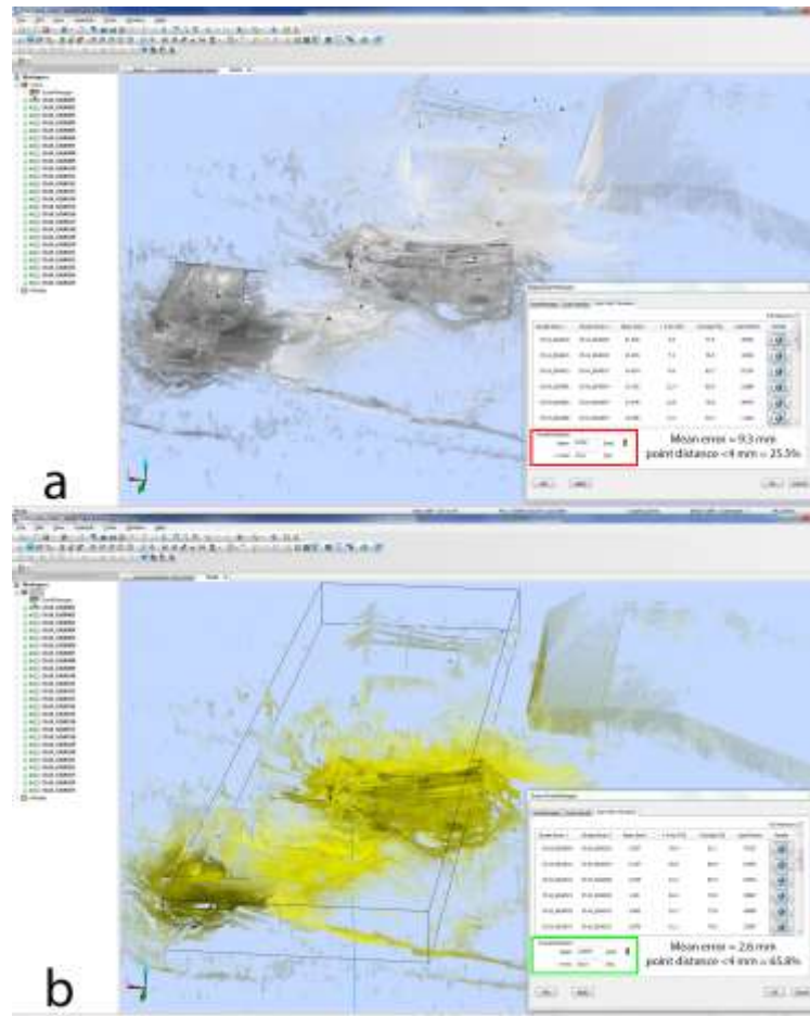
FIGURE 10 Comparison of a) top view and b) cloud to cloud target-less automatic registration of point clouds of Çatalhöyük GDA and TPC areas in FARO SCENE 5.4 showing improvement in mean error and point distance <math>< 4 \text{ mm}</math>
