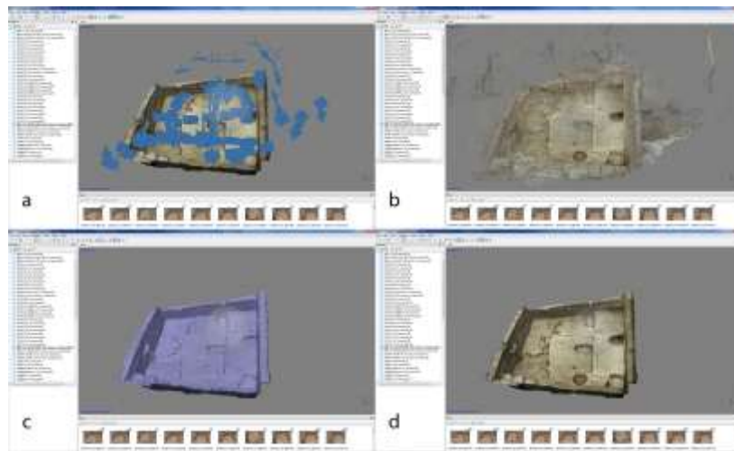
FIGURE 2 Processing of 3D data captured at the UNESCO site of Çatalhöyük, Building 89 in Agisoft Photoscan showing: a) camera positions and ground control points; b) georeferenced dense cloud; edited triangular mesh in Wireframe mode; final triangular mesh in Shaded mode
