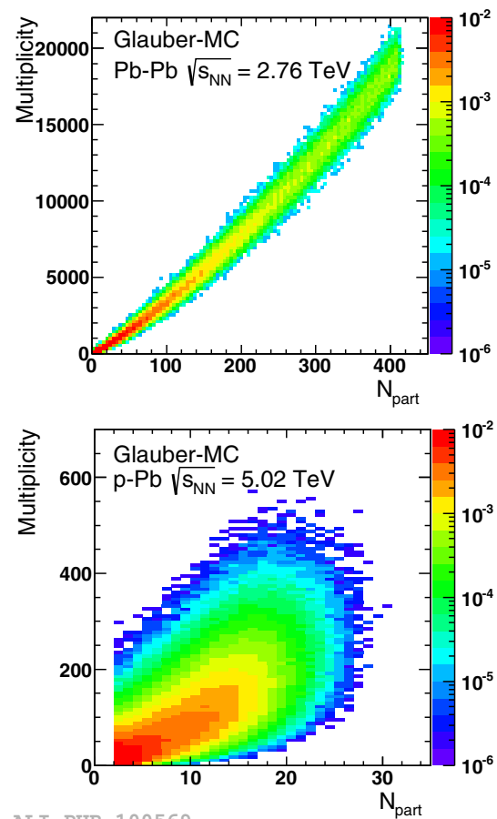
Fig. 3 Glauber-based calculations by ALICE of the correlation between forward charged-particle multiplicity (V0 detectors) and N_{part} for Pb–Pb collisions (top) and p–Pb collisions (bottom) [78]
