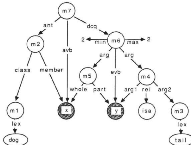
The following defines a path to find all the parts of basic level concepts (def-path parts (compose arg2- arg1 part- whole avb- ant class))
