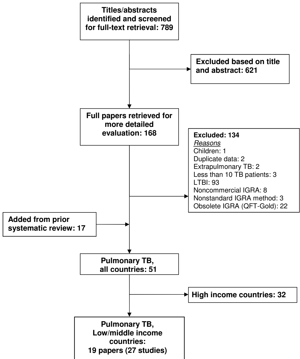
Figure 1. Study selection.
