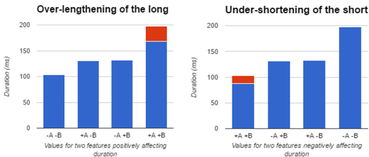
Figure 36: Two ways of understanding the Hyperadditive Lengthening Generalization. Blue bars indicate durations that would occur if the two effects combined multiplicatively with no interactions, where the longest duration (left) or the shortest duration (right) is predicted on the basis of the other three. Red bars indicate the deviation from this prediction that occurs for many pairs of durational factors, interpreted as unexpectedly long durations for either the category undergoing two lengthening effects (left) or two shortening effects (right).
