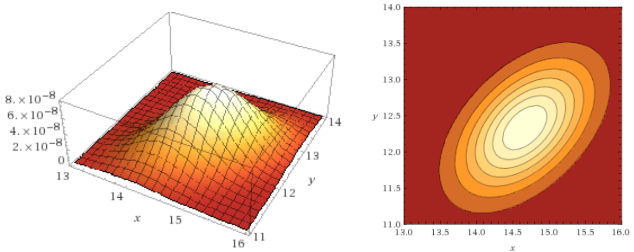
Figure 19: Maxent value as a function of F2(C) and F2(V) ( x and y , respectively) in a maxent grammar with ID(V), ID(C), and MINEFFORT, with the consonant F2 locus set to 1700 Hz, the vowel F2 target set to 1000 Hz, and all weights set to 1, following Flemming (2001). Durations are represented in hectohertz ( 10^2 Hz), rather than hertz, for visual clarity.
