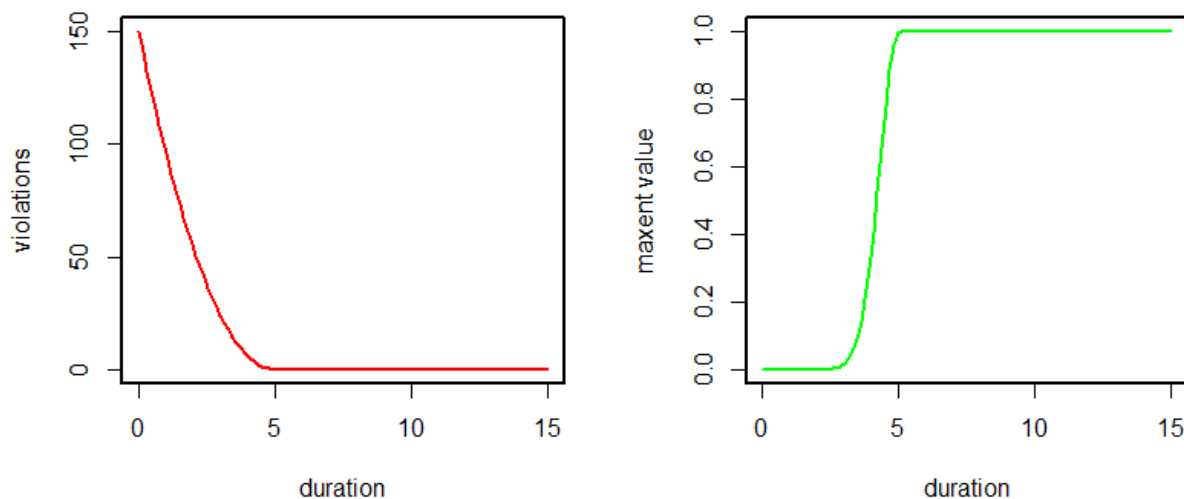
Figure 24: A pathological grammar with only a STRETCH constraint. Since the area under the maxent value curve is not defined, the probability distribution cannot be calculated.
