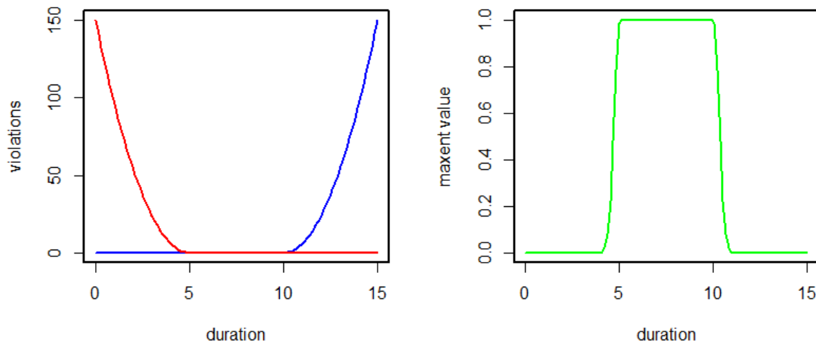
Figure 23: A “soft” window model of duration, composed of a STRETCH constraint with a shorter target (red) and a SQUEEZE constraint with a longer target (blue). Maxent values for candidates subject to both constraints are shown in green: the predicted distribution (at least without any other constraints) is uniform variation within a duration range, with a small number of outliers, depending on the constraint weights.
