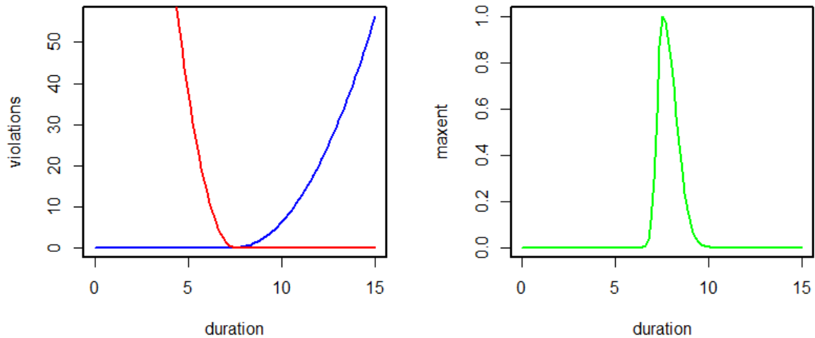
Figure 22: Violations incurred by a STRETCH constraint with a high weight (red) and a SQUEEZE constraint with a low weight (blue), and the maxent values for candidates subject to both constraints (green). The resulting distribution has a positive kurtosis / skew.
