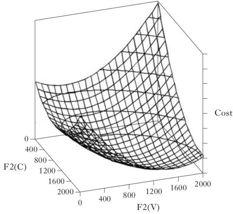
Figure 8: Figure 3 from Flemming, 2001, p. 21. Cost plotted against F2(C) and F2(V). The minimum is located at F2(V) = 1233 Hz, F2(C) = 1467 Hz.
