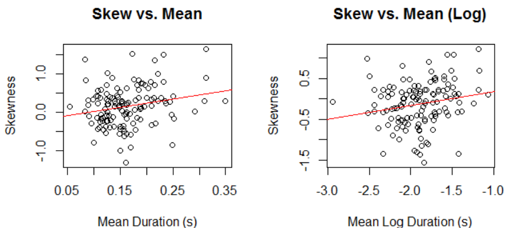
Figure 34: Skewness of samples as a function of their mean duration (left) or mean log duration (right) across the 128 experimental conditions.
