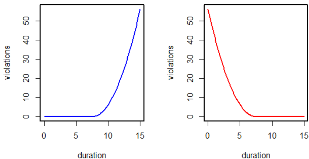
Figure 21: Hemiparabolic violation functions for STRETCH (left) and SQUEEZE (right), with weights set to 1 and targets set to 7.5.
