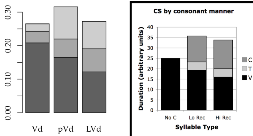
Figure 9: Figure 3.4. from Katz, 2010 (p. 112). Data from the production experiment (left) and model predictions (right) for consonant manners with high (rightmost bars) and low (center bars) vowel-recoverability coefficients. For production data, durations are in seconds. The upper bars for vowel-initial items represent closure and transition durations, in realizations where these categories are applicable.
