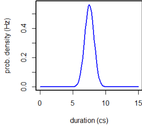
Figure 18: Predicted distribution for a single-constraint maxent grammar with a continuous candidate set.
