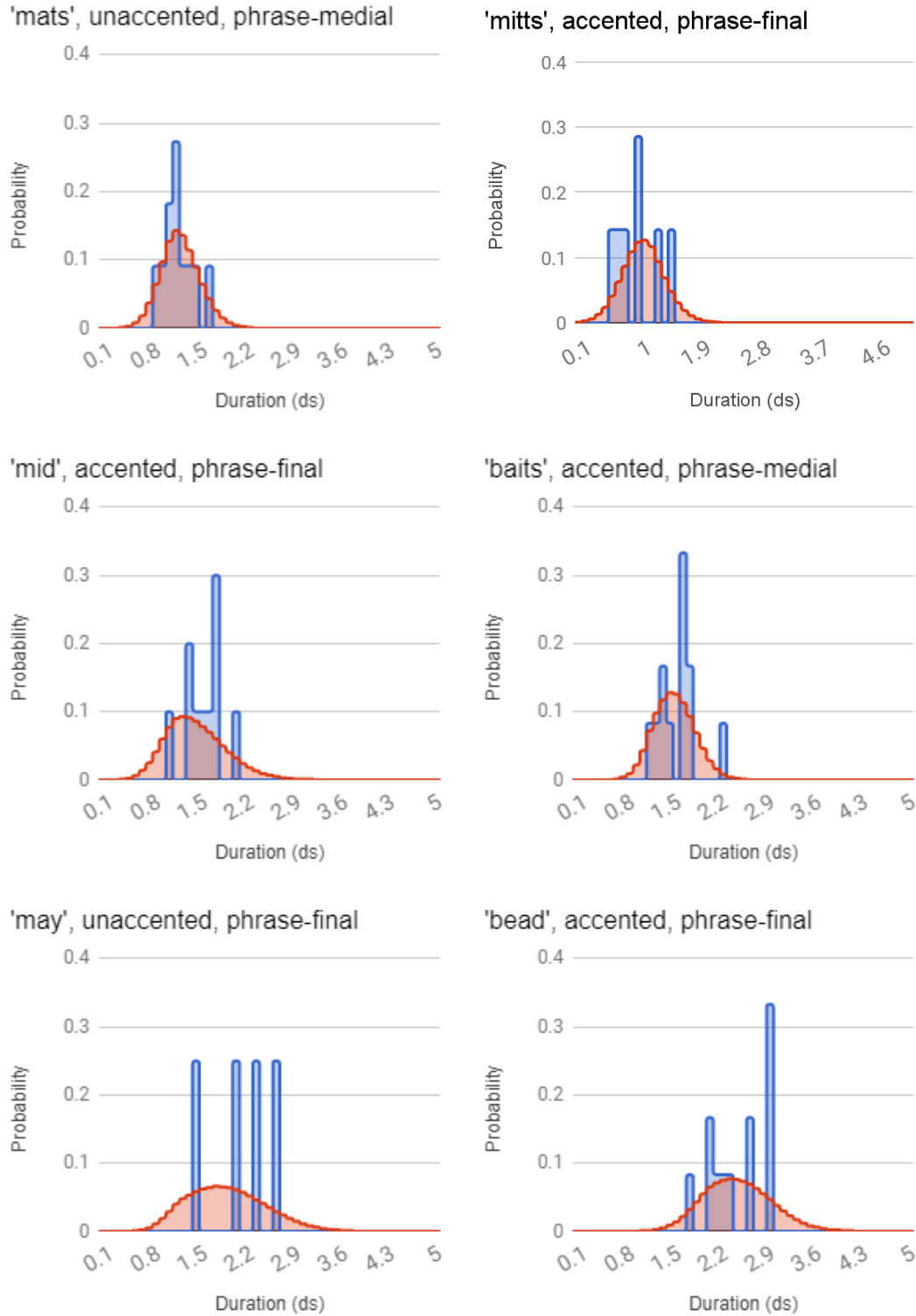
Figure 38: Predicted distributions of the S_{\text{sparse}} grammar (red), and observed histograms from the training data (blue), for six of the 128 experimental conditions.
