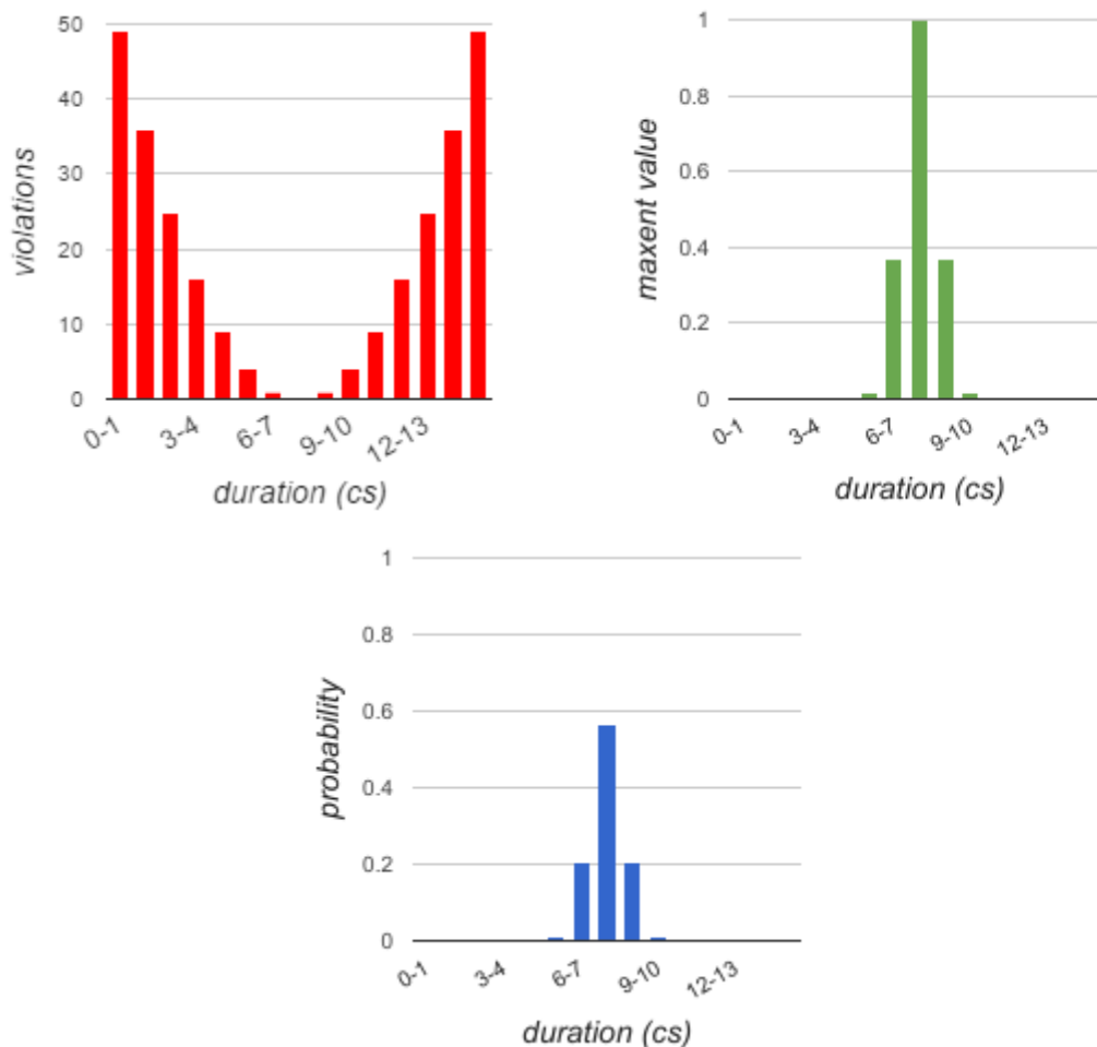
Figure 16: Violations, maxent values, and probabilities as a function of duration for a single-constraint maxent grammar with a discretized candidate set
