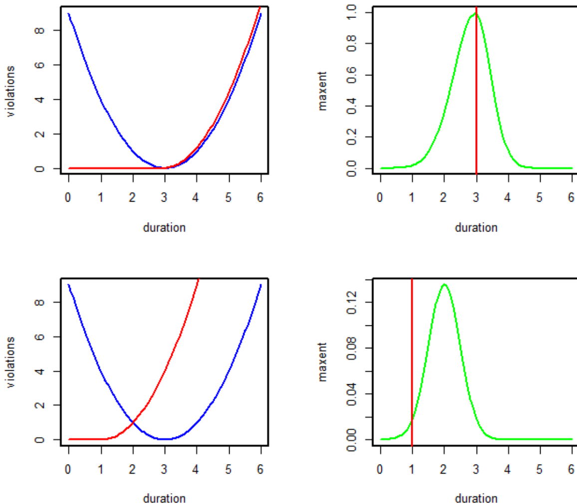
Figure 27: Violation profiles for DURATION (blue) and SQUEEZE (red), and predicted duration distributions (green) for grammars with the constraints DURATION and SQUEEZE. All weights are set to 1, the target for DURATION is set to 3, and the target for SQUEEZE is either 3 (top) or 1 (bottom), also shown as a vertical line in red.
