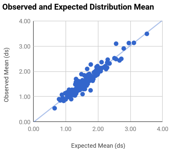
Figure 37: The means of the duration distributions predicted by the S_{\text{sparse}} grammar compared with observed sample means from the 128 experimental conditions.
