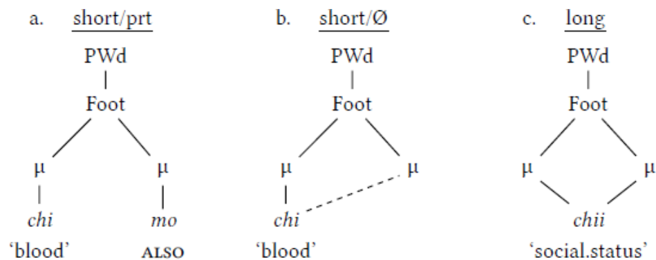
Figure 10: (8) from Braver, 2013 (p. 127). Three degrees of phonetic vowel length in Japanese.
