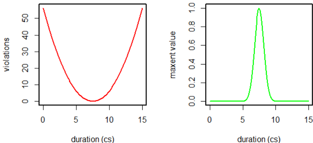
Figure 17: Violations and maxent values as a function for duration for a single-constraint maxent grammar with a continuous candidate set.
