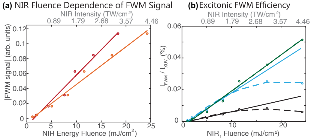
FIG. 4. Near-infrared (NIR) fluence dependence and generation efficiency of the four-wave mixing (FWM) signal. (a) The NIR fluence dependence of the strongest \text{Na}^+ core-exciton at 33.61 eV for \mathbf{k}_{\text{NIR}1} (orange) and \mathbf{k}_{\text{NIR}2} (red); spectra are collected at temporal overlap. (b) The excitonic FWM efficiency calculated for the three main core-excitations with increasing \mathbf{k}_{\text{NIR}1} fluence observed at temporal overlap. Linear (solid) and quadratic (dashed) fits; 33.27 eV = black, 33.42 eV = light blue, and 33.61 eV = green. Fluence dependence of FWM signal and excitonic efficiencies are all linear <12 \text{ mJ/cm}^2 ( <2.14 \text{ TW/cm}^2 ), NIR fluences in the 8\text{--}10 \text{ mJ/cm}^2 ( 1.43\text{--}1.79 \text{ TW/cm}^2 ) were used in the FWM studies to stay in the linear regime.
