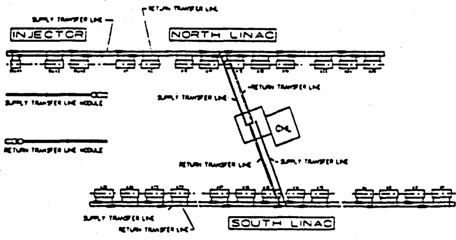
CEBAF Figure 10: Linac Transfer Line Layout (REF 10)
