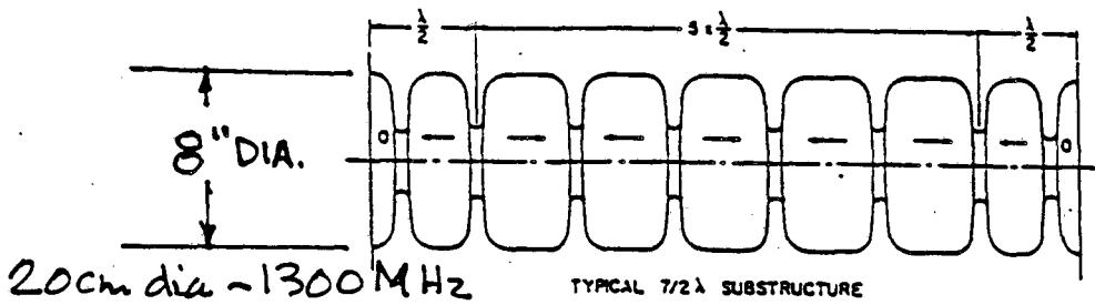
Fig. 5 Schematic of 20-foot accelerator structure and typical 7/2 wavelength (7/2 λ) sub-structures. The arrows show the relative direction of the axial electric field in the 7/2 λ sub-structure and in the individual cells. The cells which are joined by indium or lead seals are unexcited.
