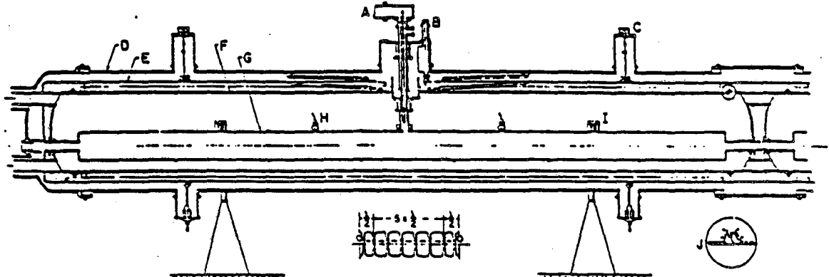
Fig. 3 Assembled 20-foot accelerator devar module. This section has end caps at one end and is connected to another module at the other end.
