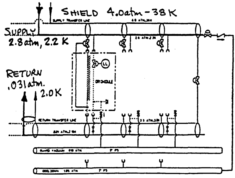
CEBAF Figure 11: Linac Transfer Line Schematic (REF. 10)
