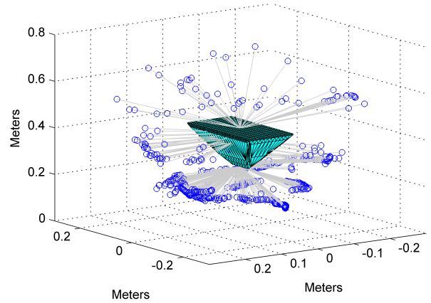
Fig. 2: Plot of a camera trajectory in 3D space. The compliant space is shown as the green tetrahedron. Each blue circle represents a camera position. At each detection an approximate shortest path (see section III-A3) can be found from camera position \mathbf{C}_w to the closest point \mathbf{O}_w on the Reduced Compliant Space Center Line.
