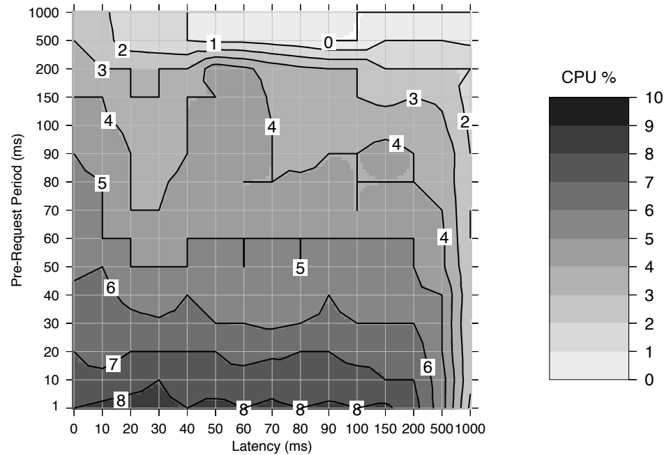
Figure 4.6 Contour map of VNC-HL CPU % for video.
