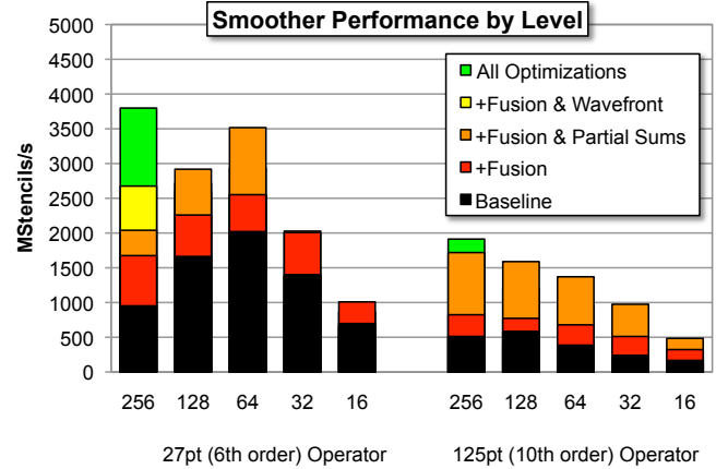
Fig. 10. Jacobi smoother performance on Edison attained with the CHiLL compiler as a function of level in the V-Cycle ( 256^3 fine grids down to 16^3 coarse grids) for the 27- and 125-point operators. Observe that the reference implementation of the memory-limited 27-point operator receives a cache boost on the coarser levels while the compute-limited 125-point does not.
