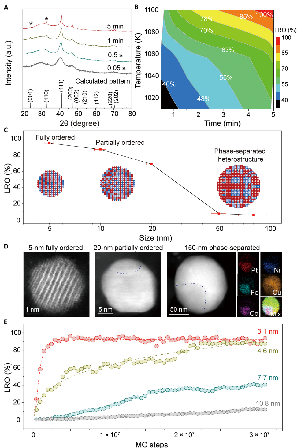
Fig. 3. The disorder-to-order phase transition process of MPEIs at the nanoscale. (A) Experimental XRD patterns of the quinary \text{Pt}(\text{Fe}_{0.7}\text{Co}_{0.1}\text{Ni}_{0.1}\text{Cu}_{0.1}) synthesized at different heating times at a temperature of \sim 1100 K and the virtual XRD pattern of the fully ordered quinary \text{Pt}(\text{Fe}_{0.7}\text{Co}_{0.1}\text{Ni}_{0.1}\text{Cu}_{0.1}) MPEI computed by the virtual XRD analysis method (40). The asterisk (*) represents the superlattice peaks of the intermetallic. a.u., arbitrary units. (B) The time and temperature dependence of the LRO of the quinary \text{Pt}(\text{Fe}_{0.7}\text{Co}_{0.1}\text{Ni}_{0.1}\text{Cu}_{0.1}) . (C) The LRO as a function of the quinary MPEI particle size. The insets schematically show the microstructural evolution as a function of the particle size. (D) HAADF-STEM images of nanoparticles of increasing size ( \sim 5 , 20, and 150 nm), in which the smallest nanoparticle features an ordered structure, while the larger particles become increasingly disordered, corresponding to the schematics in (C). EDX mapping of the 150-nm particle shows its phase-separated structure. (E) The simulated LROs of different-sized nanoparticles (3.1, 4.6, 7.7, and 10.8 nm) as a function of the MC simulation steps.
