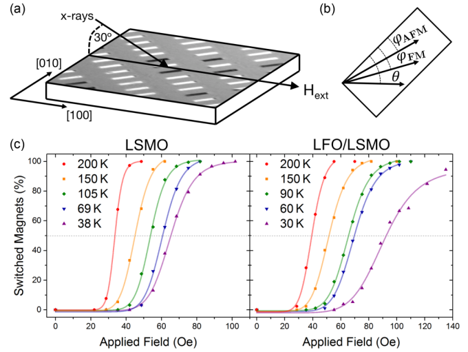
FIG. 2. (a) XMCD image of a partially switched ((110)-oriented, LSMO single layer at 105 K after applied field of 49 Oe) micromagnet array combined with schematic of the X-PEEM experimental setup depicting the incident x-ray angle, micromagnet orientation, and applied field direction. (b) Angles for applied field H_{\text{ext}} , FM spin axis \varphi_{\text{FM}} , and AFM spin axis \varphi_{\text{AFM}} defined relative to the long axis of the individual micromagnets. (c) Percentage of micromagnet array switched vs applied field for the LSMO single-layer (left) and LFO/LSMO bilayer (right) samples at temperatures between 30 and 200 K. Solid lines are normal cumulative distribution function fits, and the intersection with the horizontal dashed line corresponds to the field where 50% of micromagnets have switched.
