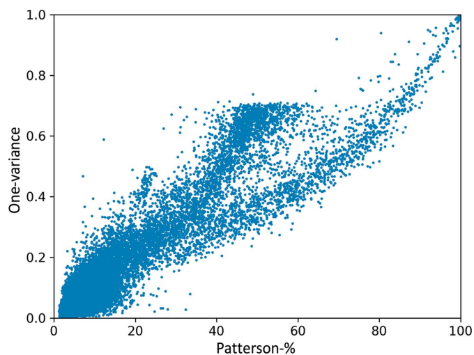
Figure 6 Scatter plot showing the distribution of refined TNCS epsilon factor one-variance (variance about 1; equation 6) for all cases with pdb-TNCS(20°). Data resolution range 5–10 Å.
