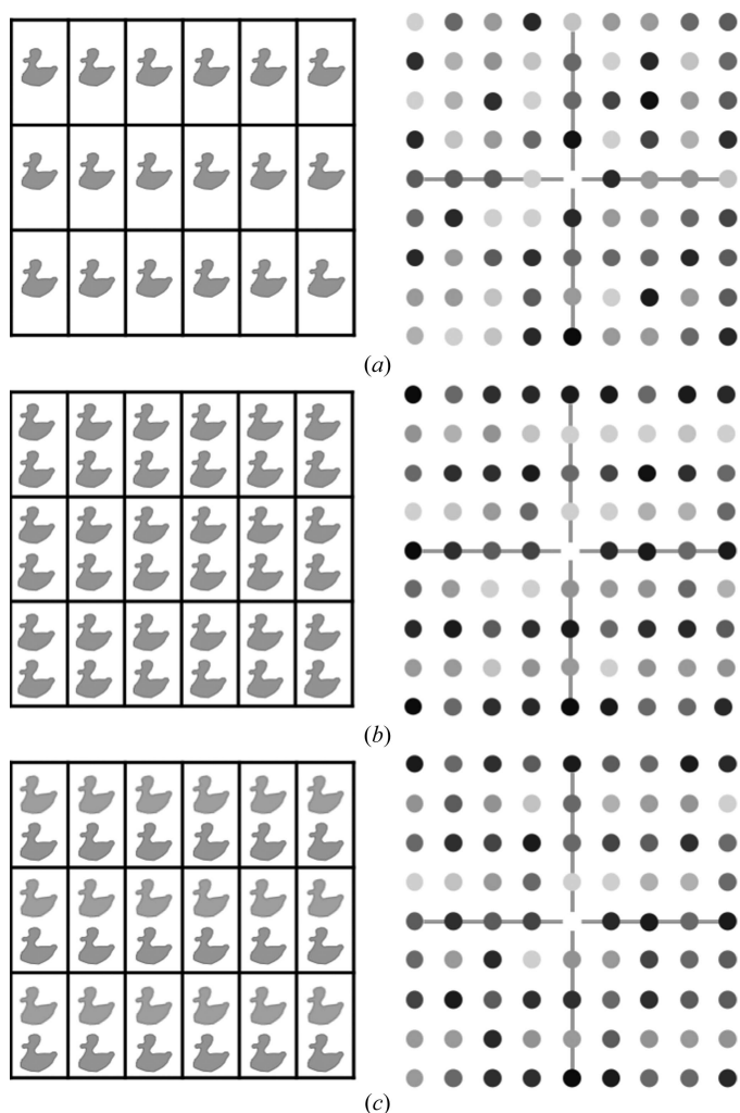
Figure 1 Modulation of diffraction intensities for a molecule (represented by a duck) with significant anomalous scattering, so that Friedel's law is not obeyed. The arrangement of molecules in the crystal is shown with the h0l layer of reciprocal space (right). (a) A crystal without TNCS and intensities with no modulation. (b) A crystal with TNCS between two molecules, shifted by a vector close to half the y -axis lattice translation. The intensities show weaker than average intensity reflections in the odd rows and stronger than average intensities in the even rows. (c) A crystal with TNCS between two molecules, shifted by a vector close to half the vertical lattice translation and with a 20^\circ rotation. The intensities show the same pattern of intensity modulations as in (b), but not as pronounced.
