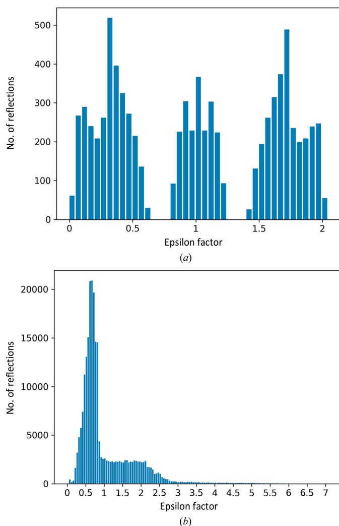
Figure 5 Histograms showing the distribution of refined TNCS epsilon factors for (a) PDB entry 2cc0 with \sigma_1^2 = 0.63 for TNCS 2 (Taylor et al. , 2006) and (b) PDB entry 4n3e with \sigma_1^2 = 0.61 for TNCS 7 (Sliwiak et al. , 2014).
