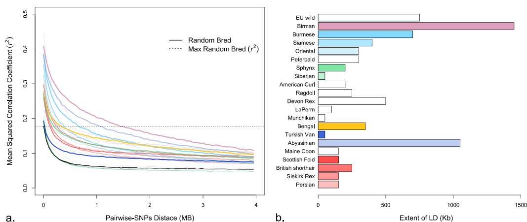
Figure 4. Genome-wide estimate of linkage disequilibrium (LD) of cat breeds. (a) Decay of LD ( r^2 ) at different bins of inter-SNP distances. LD decay of selected population is shown as a color (see (b) for key to colors) and remaining populations are shown in gray. Solid black decay line corresponds to the random bred population, to which all breed populations are compared. Horizontal dotted line represents the maximum of r^2 value in random bred population and the point of comparison between populations (the point of LD < 50 Kb). (b) Extent of LD (Kb) where the r^2 value reaches that of random bred population.
