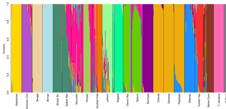
Figure 3. Population structure plot (K = 19) of twenty cat breeds and two wildcat populations. faststructure was used to examine the same cat populations as described for the MDS analyses. Cat breeds with the same colors indicate admixture and shared ancestry/cross-breeding. For examples, Peterbalds are derived from Siamese and Oriental lines and several breeds have been developed from Persian lineages, such as Munchkins and Scottish Fold, to obtain brachycephalic head structure.
