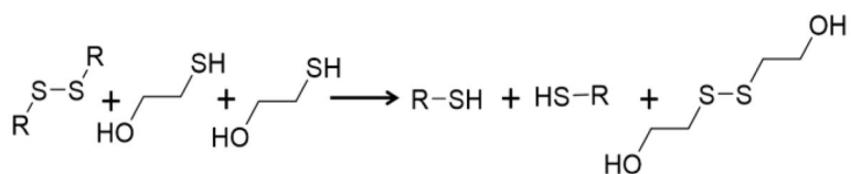
Scheme 1. Disulfide chemical reduction mechanism
