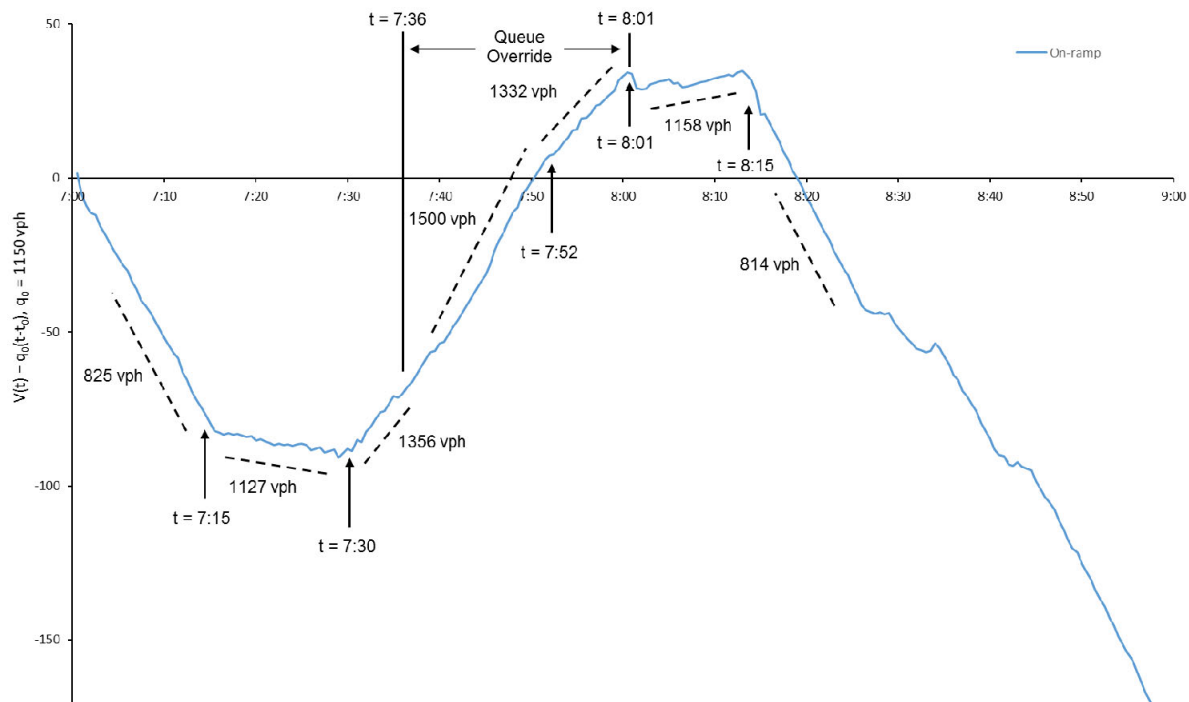
Figure 3. May 10, 2016: O(t) curves for McKee Rd. on-ramp.
