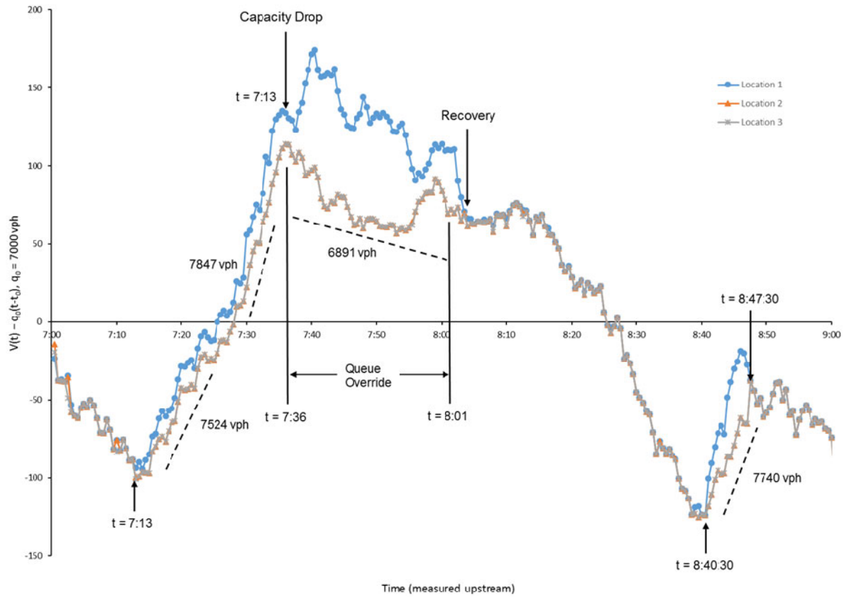
Figure 2. May 10, 2016: O(t) curves for locations 1 through 3.
