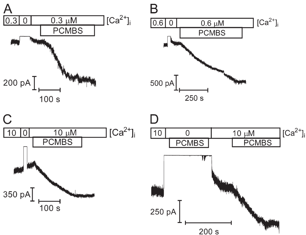
Figure 1. PCMB5 increases KCa3.1 steady-state current. Macroscopic current records from KCa3.1 channels heterologously expressed in HEK cells to determine sensitivity to PCMB5. PCMB5 (500 \mu\text{M} ) was added to inside-out patches excised in 0.3 (A), 0.6 (B), and 10 \mu\text{M} (C) \text{Ca}^{2+}_i after the establishment of steady-state current level. PCMB5 washout lasted at least 1 min to ensure channel activation was due to covalent binding, rather than an indirect interaction between channel and compound. (D) KCa3.1 current record demonstrating that PCMB5 cannot activate the channel in the absence of \text{Ca}^{2+}_i . PCMB5 can only increase current when the channel is in the open state. The patch was initially excised in 10 \mu\text{M} \text{Ca}^{2+}_i , followed by the addition of a \text{Ca}^{2+}_i -free solution, and then a \text{Ca}^{2+}_i -free solution+PCMB5 (500 \mu\text{M} ) was added to the bath solution. PCMB5+ \text{Ca}^{2+}_i -free solution was washed out with 10 \mu\text{M} \text{Ca}^{2+}_i to reactivate the channel. After reaching a steady-state current level, PCMB5 (500 \mu\text{M} ) was reapplied to the patch, resulting in channel activation.
