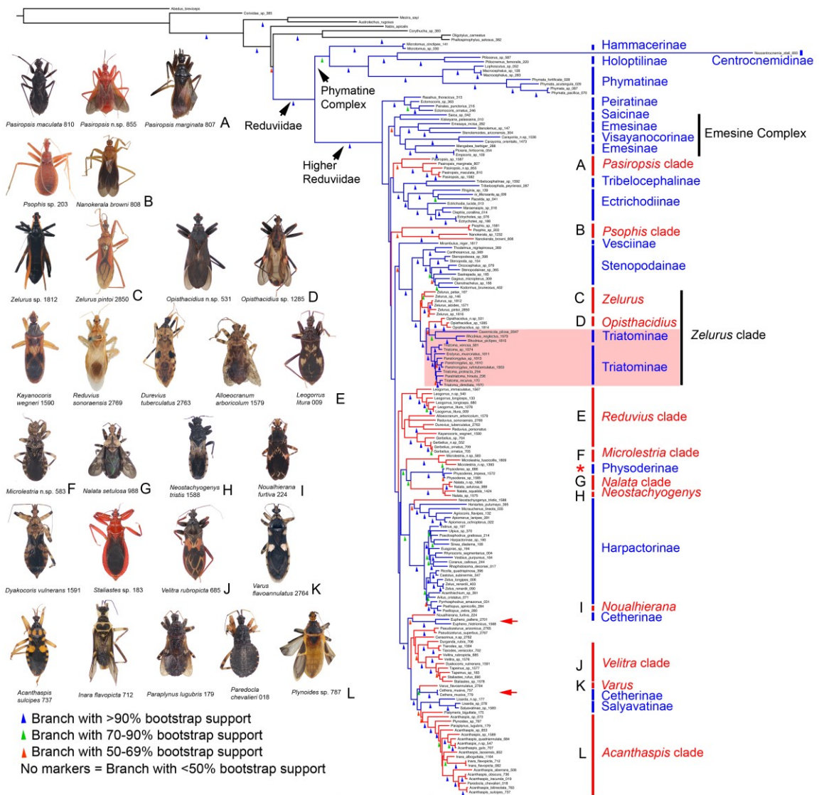
Figure 1.1. Maximum Likelihood phylogram with representative habitus images of reduviine clades. Best tree (score = -83447.290932) based on RAxML analysis of 178 taxa using a partitioned molecular dataset of 5 gene regions (16S, 18S, 28S D2, 28S D3-D5, Wg) aligned with MAFFT G-INS-i. Bootstrap values are indicated on branches by colored triangles according to support strength (explained by inset). Reduviinae lineages are indicated as red branches and remaining reduviids as blue while outgroup taxa are black. Habitus images of Reduviinae species with RCW specimen ID numbers are grouped (A-L) according to the 11 separate reduviine clades. The shaded red box highlights members of the hematophagous Triatominae, here shown
