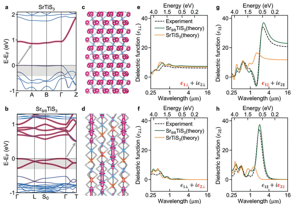
Figure 3. Electronic structure and optical properties of modulated \text{Sr}_{9/8}\text{TiS}_3 . a,b) Orbital-projected band structures for hypothetical stoichiometric \text{SrTiS}_3 (a), and modulated \text{Sr}_{9/8}\text{TiS}_3 (b). The thicker lines highlighted in red correspond to the contribution from Ti- 3d_{z^2} states. The Fermi energy is set to 0 eV. c,d) Spatial distribution of the valence electrons below the Fermi energy (shaded in gray in (a) and (b)), showing S-3p character in \text{SrTiS}_3 (c) and Ti- 3d_{z^2} character in \text{Sr}_{9/8}\text{TiS}_3 (d). The isosurface is set to an electron density of 0.004 \text{ e} \text{ \AA}^{-3} . e–h) Calculated complex dielectric function for polarization perpendicular ( \epsilon_{\perp} ) and parallel ( \epsilon_{\parallel} ) to the c -axis of the hypothetical stoichiometric \text{SrTiS}_3 and modulated \text{Sr}_{9/8}\text{TiS}_3 , compared to the experimental results (black dashed line). The index i = 1 represents the real part of the dielectric function and 2 represents the imaginary part.
