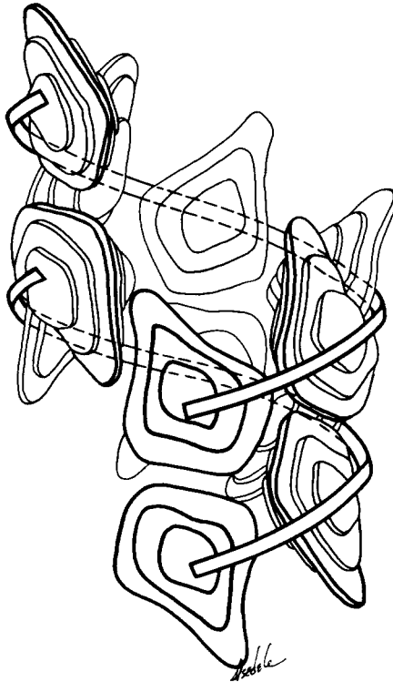
Fig. 6. A proposed model for the structure of one turn of the gene 5 protein–DNA double helix. This arrangement arises by opening the disk structure seen in Figure 5 between any two adjacent dimers and displacing the free ends along the unique axis direction. The stacking of these "lockwasher" units results in a double helix structure having a sixfold screw axis with perpendicular dyads, 12 gene 5 monomers per turn, and dimensions consistent with the helices observed by electron microscopy. The two DNA single strands are spooled around this spindle of gene 5 protein.
