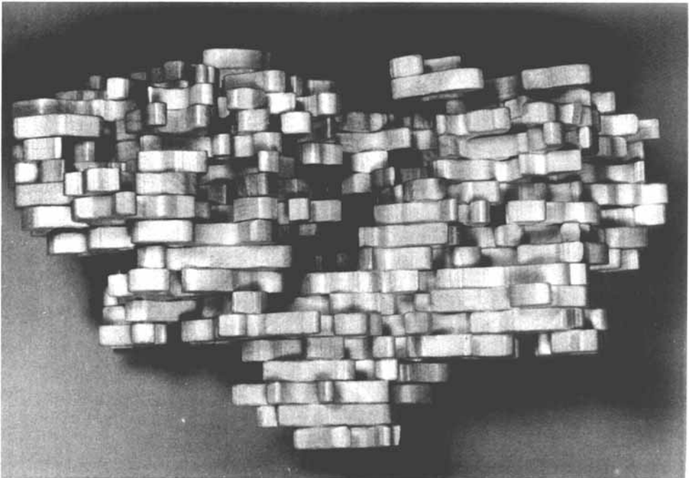
Fig. 4. A photograph of a three-dimensional model representation of the gene 5 dimer based on the structure derived from X-ray diffraction analysis. The postulated binding regions for the DNA single strands lie beneath the thick mass of density and are separated in the dimer by about 25 Å.
