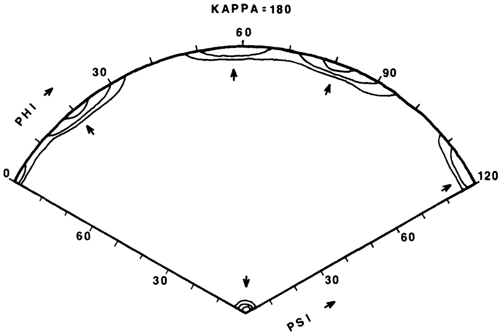
Fig. 3. The \kappa = 180^\circ section of the rotation function of the crystals of complexes between the gene 5 protein and d-(GGTAAT). All of the peaks along \psi = 90^\circ are of high magnitude with respect to the crystallographic symmetry peak, and all represent local, noncrystallographic symmetry elements present in the crystals.
