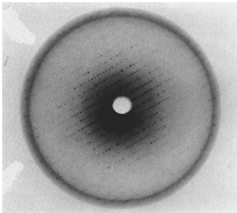
Fig. 2. Precession X-ray diffraction photograph of the zero level of the 0kl zone of reciprocal space of the P3_1 crystals of gene 5 protein complexed with d-(GGTAAT). These crystals grow to large size and diffract strongly to at least 3.0 Å in precession photographs.
