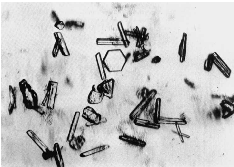
Fig. 1. Low-power light microscope photograph of the hexagonal plate habit of the complex between gene 5 protein and d - pCpTpTpC . These crystals have been observed to exist in the same sample with rhombic plates.
