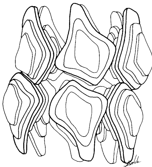
Fig. 5. A proposed model for the asymmetric unit common to the four crystal forms we have so far analyzed. The arrangement is a circle, or disk, having 622 point group symmetry formed by joining the two ends of a linear array of six gene 5 protein dimers, each of which possesses an inherent dyad, to produce closure. The upper hexagon of monomers will bind a single strand of DNA running in one direction and the bottom level a strand running in the opposite direction. The disk has a diameter of about 100 Å and a height of about 80 Å. We believe the DNA binding region of each monomer to be directed toward the outside of the circle.
