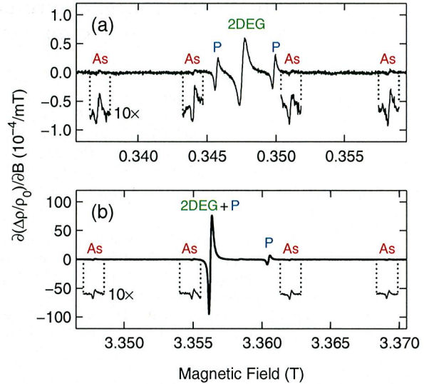
FIG. 2: (a) EDMR spectra obtained in X- and (b) W-band. The 2DEG, phosphorus (P) and arsenic (As) resonances are indicated along the traces. Sections of the EDMR spectra are magnified by 10 \times and offset for clarity. The gate bias was 0.3 V and the drain bias was 40 mV in both measurements.
