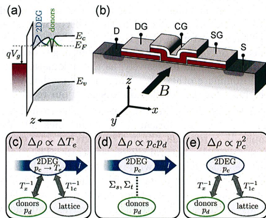
FIG. 1: (a) Energy-band diagram of the MOS system showing the overlap of the 2DEG and donor electron wavefunctions. (b) Schematic of the aFET used, where the drain (D) and source (S) are separated by three gates (DG, CG and SG). 31 P donors are present under all three gates while 75 As donors reside under the CG region only. (c–e) Three possible EDMR mechanisms affecting the 2DEG current I (blue arrow), and the expected change in resistivity \Delta\rho associated with each mechanism: (c) bolometric heating, (d) spin-dependent scattering and (e) polarization transfer. The grey arrows represent energy transfer between the systems, while the dashed line in (d) represents elastic scattering. See text for the definition of symbols.
