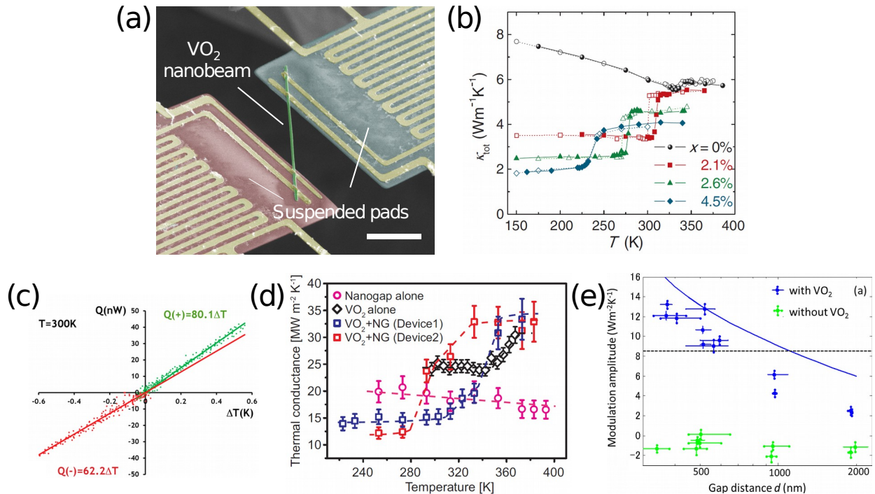
Fig. 6.5 (a) SEM image of a suspended-microdevice, for thermal conductivity measurements, consisting of two T-sensing pads (red for high T and blue for low T) and a VO 2 nanobeam (green) [51]. Scale bar, 10 \mu\text{m} . (b) Experimentally measured total thermal conductivity of W_xV_{1-x}O_2 nanowires [51]. (c) Heat flow (Q) as a function of \Delta T across a tapered VO 2 nanowire at 300 K. Different signs (+) and (-) of Q represent different directions of heat transfer. Thermal conductance, i.e. the slope Q/\Delta T , differs depending on the direction of the heat flow [214]. (d) Temperature dependence of cross-plane thermal conductance of solid-state nanomechanical thin-film structures having nanogap (NG) alone, VO 2 film alone, and VO 2 plus NG (Device1 and Device2) [213]. (e) Modulation amplitudes (defined as the value of heat transfer coefficient at 295K (M1) minus that at 325K (R)) measured by radiative heat transfer through the nanogap between a SiO 2 emitter and W_xV_{1-x}O_2/\text{SiO}_2 receiver [215].
