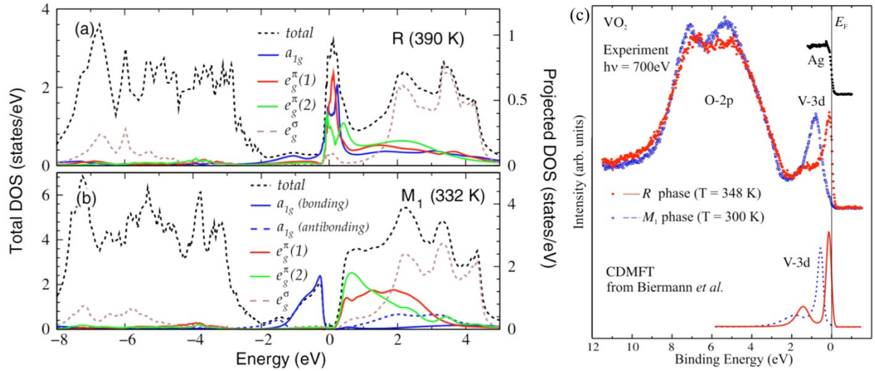
Fig. 2.3 (a, b) Total and orbital-projected electron DOS for M_1 and R phases, as obtained from DFT+DMFT [29]. (c) X-ray photoemission spectra of rutile (red) and monoclinic (blue) phases below the Fermi level [32]. The theoretical curves in (c) are c-DMFT calculation results from [27].
