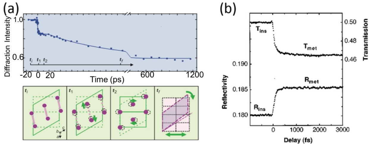
Fig.3.3 (a) The diffraction intensity change explained by stepwise structure distortion under the ultrafast electron diffraction experiment, with the corresponding stepwise structure distortion plotted below [67]. (b) Reflectivity and transmission change under ultrafast photo-excited phase transition experiment [66].
