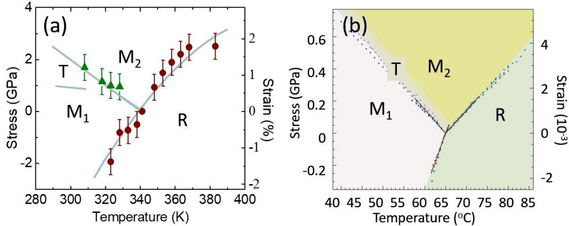
Fig. 4.1 (a) Uniaxial (along c_R -direction) stress – temperature phase diagram of \text{VO}_2 [84] mapped by imaging domain structure of bent \text{VO}_2 nanobeams [78]. The small stripe of T phase between the M1 and M2 regions were obtained from Raman spectroscopy of bent \text{VO}_2 nanobeams [88]. (b) A refined measurement of the phase diagram at small strains identifies the triple point of M1, M2 and R phases converging to zero strain [11]. Note that most of the samples measured have sizes larger than hundreds of nm, so no size effect is expected in the phase diagram.
