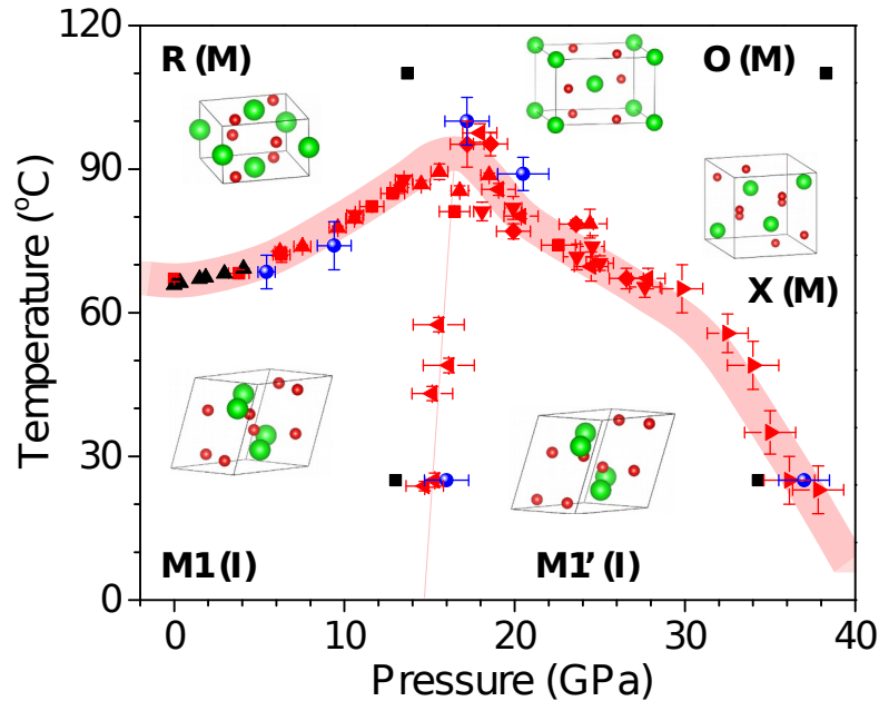
Fig. 4.2 Hydrostatic pressure - temperature phase diagram of \text{VO}_2 [91]. I and M in parenthesis represent insulating and metallic phases, respectively. Insets are the simulated atomic structures of each phases of \text{VO}_2 (V: green atoms, O: red atoms). The red and blue data points on the phase boundaries are obtained from Raman and electrical measurements, respectively, and different shapes of symbols represent different samples. The black square data points are determined by XRD extracted from Ref. [89]. The black triangle data points are from Ref. [86].
