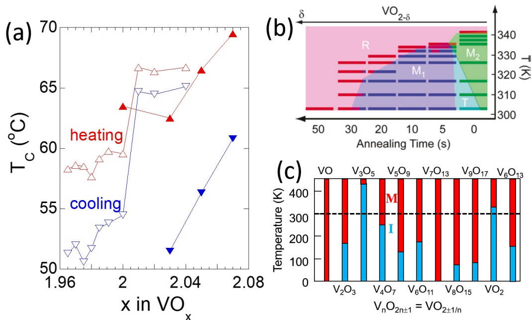
Fig. 4.4 (a) MIT temperature of \text{VO}_2 as a function of oxygen non-stoichiometry [96]. (b) Raman-determined phase diagram of non-stoichiometric \text{VO}_2 obtained by thermal annealing under reducing conditions
