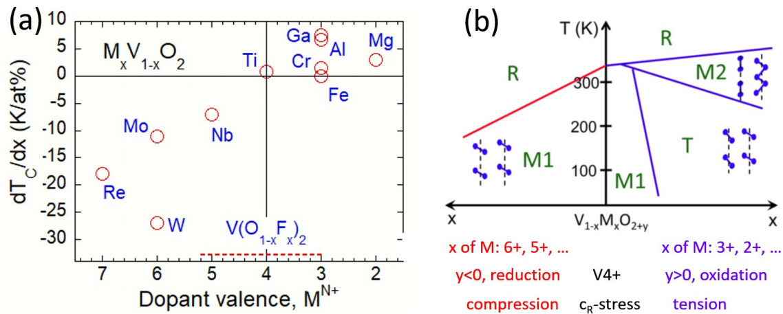
Fig.4.6 (a) Changing rate ( dT_c/dx ) of the MIT temperature with dopant atomic fraction ( x ) for cation substitutional doped \text{VO}_2 . The data of dT_c/dx = -32 K/at% for anion F-doped \text{VO}_2 is also indicated with a dashed line [114]. Note that the real valence state of the dopant was not directly confirmed as many of the dopants are multi-valent (e.g., Fe, Cr). (b) A schematic phase diagram of \text{VO}_2 for doping, non-stoichiometry, and uniaxial stress [133].
