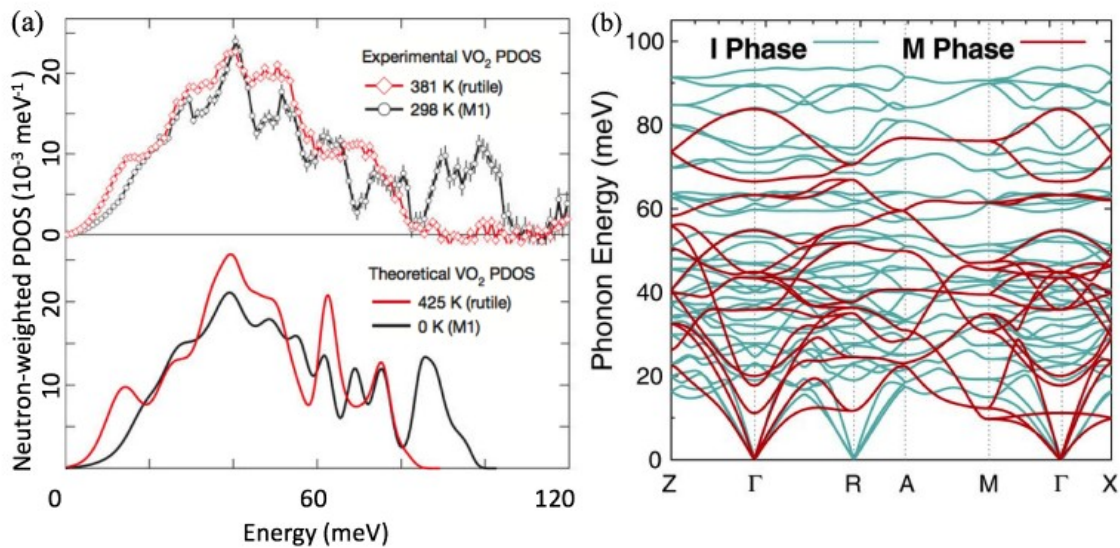
Fig.3.2 (a) Phonon density of states in R and M1 phases, from inelastic neutron scattering measurement and DFT based calculations [25]. (b) Calculated phonon spectrum for M1 and R phase [51].
