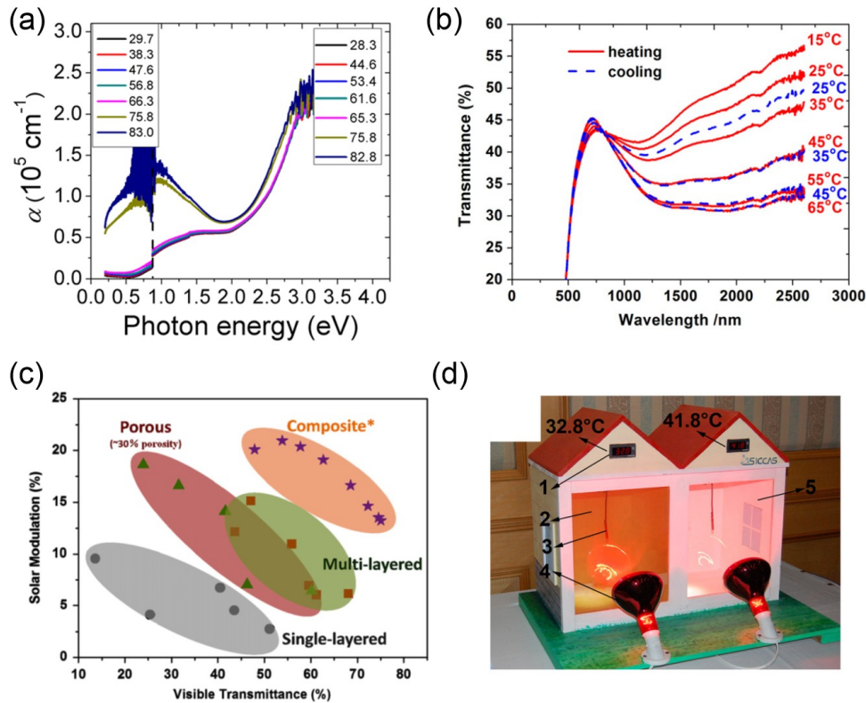
Fig. 6.2 (a) Absorption coefficient of a VO 2 thin film (deposited on sapphire by PLD) at different temperatures (in units of °C) [109]. (b) Dependence of transmittance spectra on temperature for a W-doped VO 2 film [143]. (c) Thermochromic performance of different structures based on VO 2 thin films [143]. (d) A model house with window coated by W-doped VO 2 film (left) versus with a blank glass window (right). 1, Temperature monitor; 2, glass coated by W-doped VO 2 ; 3, temperature sensor; 4, infrared lamp; and 5, blank glass [143].
