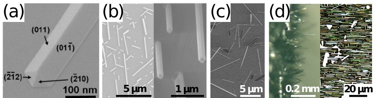
Fig. 5.3. (a) SEM image showing a VO_2 nanowire with Miller indices of its facets at both the tip and the side [166]; (b-f) VO_2 nanowires grown via VTM on various substrates: (b) SEM images of nanowires grown on a c-cut (left panel) and a r-cut (right panel) sapphire substrates [166], (c) SEM image of laterally grown, randomly oriented nanowires on silicon (110) [167], (d) optical images of free-standing nanowires grown on a rough quartz substrate (left panel) [163] and laterally grown nanowires on an a-plane quartz surface (right panel) [168].
