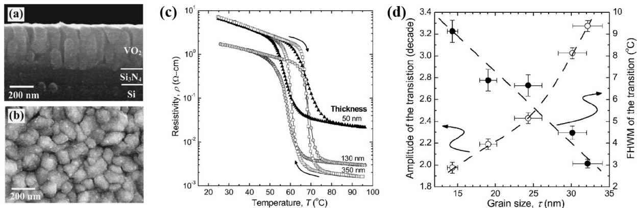
Fig.5.1 (a) Side view and (b) top view of a 350 nm thick VO 2 film deposited by magnetron sputtering [146]. (c) MIT of VO 2 thin films with different thicknesses. (d) Dependence of amplitude and FWHM of transition temperature of the MIT of VO 2 thin films on grain size [146].
