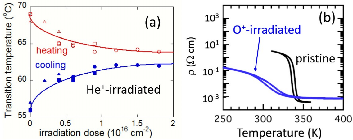
Fig.4.5 (a) Heating and cooling MIT temperatures as a function of the dose of 3 MeV \text{He}^+ irradiation on single-crystal, strain-free \text{VO}_2 nanobeams, showing closing of the hysteresis loop at high vacancy and interstitial defect densities [17]. (b) Resistivity - temperature characteristics of a \text{VO}_2 thin film after high ( 2 \times 10^{15} \text{ cm}^{-2} ) dose irradiation of 110 keV \text{O}^+ ions [111]. The MIT quality and the MIT temperature are both reduced.
