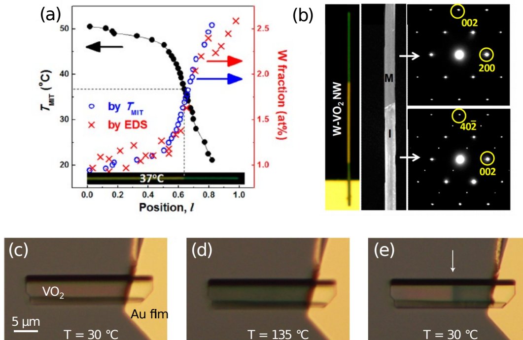
Fig. 5.4. (a) Local MIT temperature (left axis) and tungsten fraction (right axis) of an axially graded-doped W_xV_{1-x}O_2 nanowire. The horizontal axis is positioned along the graded-doped nanowire from the center ( l = 0 ) to the tip ( l = 1 ). The inset shows optical image of the analyzed nanowire at 37 °C as an example. (b) Optical (left panel) and TEM (middle panel) images with the SAED patterns (right panels) corresponding to the metallic (R, upper-right panel) and insulating (M1, lower-right panel) domains [162]. (c-e) Optical images showing hydrogenation of VO 2 : a VO 2 micro-crystal in H 2 atmosphere at (c) 30 °C, (d) 135 °C, and (e) at 30 °C (after cooled down from 135 °C) [98]. The right bright region is gold film deposited to cover the end of the VO 2 crystal. A domain boundary, indicated by the arrow in (e), implies that the hydrogen doping fraction varies axially along this crystal.
