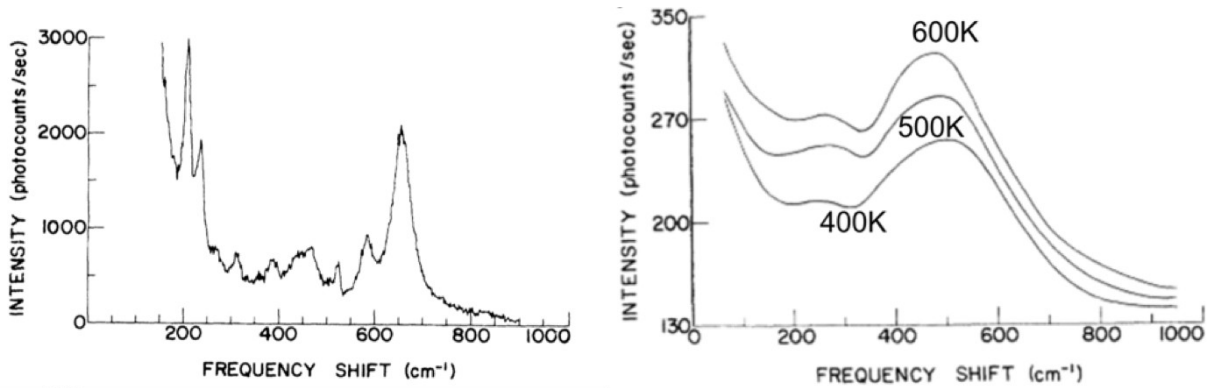
Fig. 3.1 Unpolarized Raman spectra of low temperature M1 phase at 300K (a) and of high temperature VO 2 R phase at 400 K, 500 K and 600 K (b) [58].
