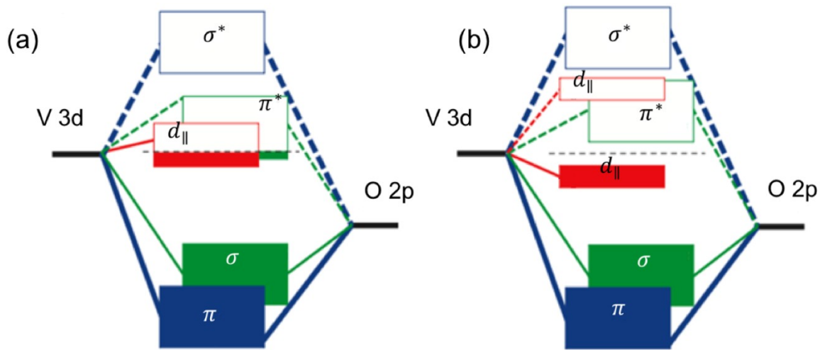
Fig. 2.2 Graphic of VO_2 electronic band structure in the R (a) and M1 (b) phase [19].
