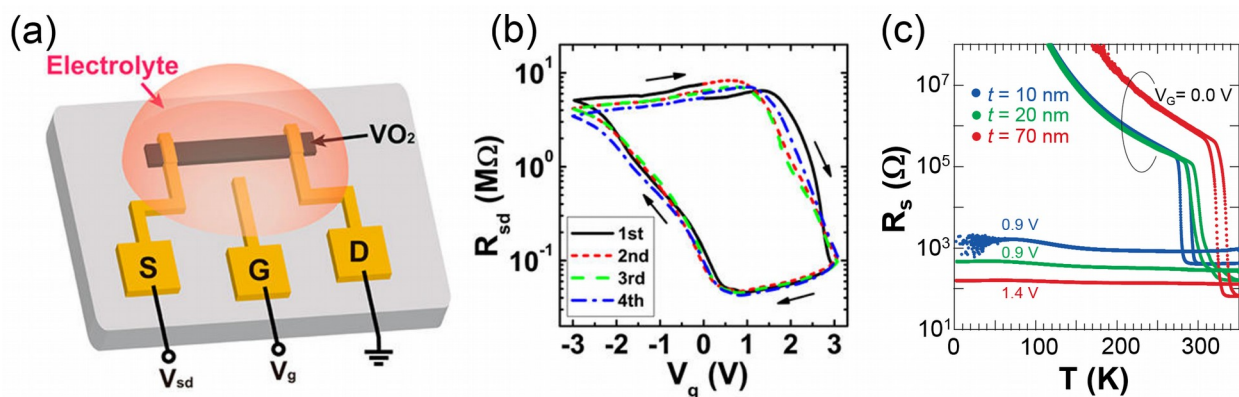
Fig. 6.3 (a) Schematic of a liquid-gated FET configuration based on single-crystal VO 2 nanobeam [189]. (b) Source-drain resistance of a VO 2 nanobeam as a function of gate voltage for several scans [189]. (c) Temperature dependence of sheet resistance for VO 2 thin films with different thicknesses at two gate voltages, showing E-field induced metallic states [93].
