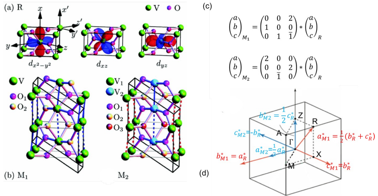
Fig.2.1 (a) Unit cell of rutile phase with d orbitals in different polarization directions [18]. (b) Unit cell of Monoclinic M1 and M2 phase of VO2 [18]. (c)
