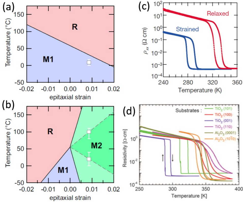
Fig.4.3 (a) Proposed phase diagram and experimental data of biaxially strained (001) R VO 2 films where the strain is equal in a R and b R directions [92]. (b) The same for anisotropically strained (100) R VO 2 films plotted as a function of the b R strain where the c R strain is fixed to be 4.35 times higher. (c) Experimentally measured MIT for VO 2 films pseudomorphically strained (when thickness is 10 nm) or relaxed (when thickness is 70 nm) grown on (001) TiO 2 substrates [93]. (d) Experimentally measured MIT characteristics of VO 2 films grown with different thicknesses on different substrates [95].
