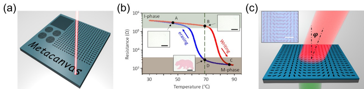
Fig.6.6 (a) Schematic of laser writing different photonic patterns on a metacanvas [218]. (b) Temperature-dependent resistance of a VO 2 film, where the transition temperature ( T_d ) is denoted by a vertical dashed line. Inset A and B: un-patterned VO 2 film (all in I-phase). Inset D: the VO 2 film (global temperature kept at T_d ) is laser-written with a pattern of a bear in the M-phase [218]. (c) Schematic of a meta-canvas programmed as a beam steerer with a steering angle \varphi . Inset: optical image of the beam steering phase array compiled on the VO 2 metacanvas (Scale bar is 10 \mu\text{m} in Inset) [218].
