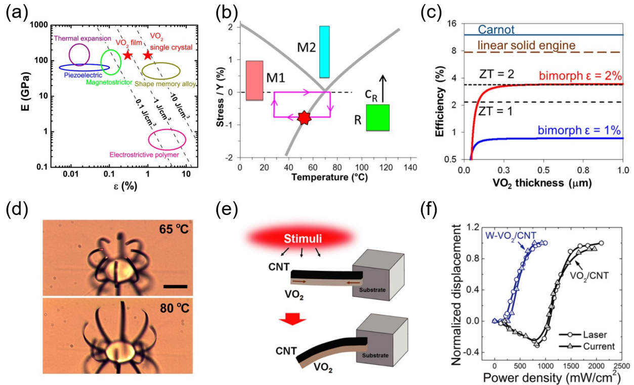
Fig. 6.4 (a) Comparison of work densities of various actuation materials [203]. (b) Phase diagram ( C_R stress vs temperature) of VO_2 . The rectangular loop shows a possible cycle of the solid engine, and the red star is the point where the work is done [197]. The rectangular boxes show schematically the size and shape of the single crystal in the three phases, respectively. (c) Calculated energy efficiency of a VO_2 -based linear solid engine and bimorph solid engines for transformation strain of \epsilon = 1\% (M1-R) and 2\% (M2-R) [197]. (d) Microactuator with a “palm” structure, showing the fingers closed at 65^\circ\text{C} and open at 80^\circ\text{C} . Scale bar, 50\ \mu\text{m} [203]. (e) Schematic of a flexible VO_2/\text{CNT} bilayer actuator [204]. (f) Comparison of the performance of bilayer actuators based on W-doped and undoped VO_2 thin film under light illumination [204].
