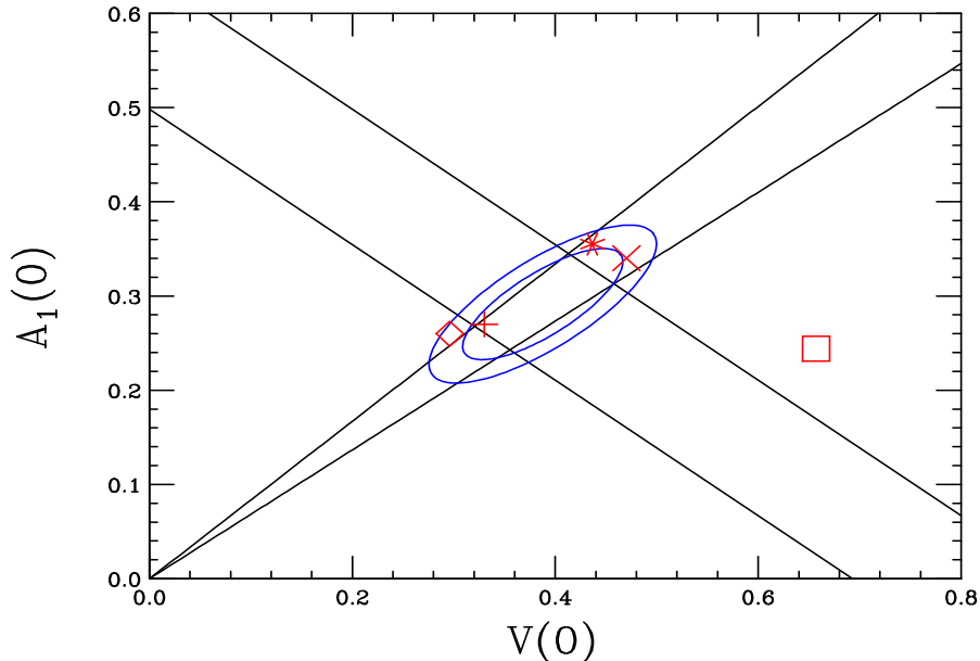
Figure 1: Constraints on the semileptonic form-factors V(0) and A_1(0) from B \rightarrow K^*\gamma data plus HQSS (thicker band) together with the relation from the LEL (thinner band). The ellipses correspond to 68% and 90% confidence level intervals. Central values of model predictions are also shown and correspond to BSW [12] (vertical cross), ISGW2 [13] (diamond), MS [14] (star), LCSR [15] (diagonal cross) and LW [16] (square), respectively.
