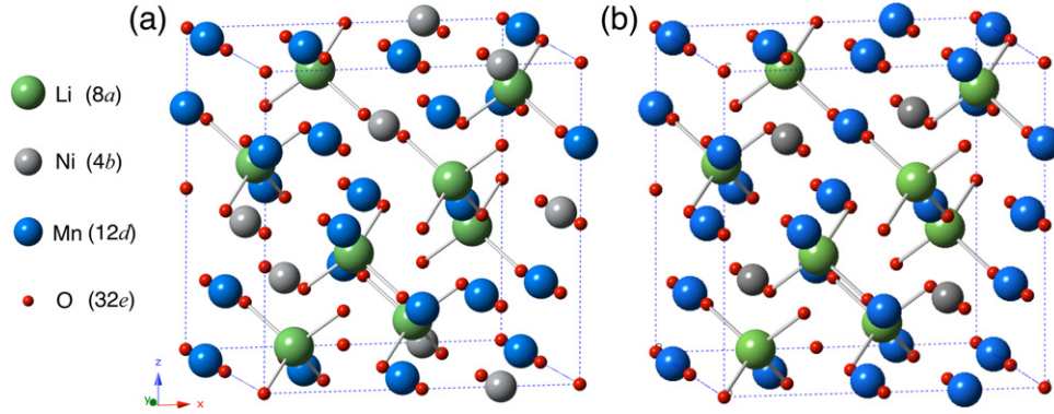
Figure 1. Unit cell of the \text{LiNi}_{0.5}\text{Mn}_{1.5}\text{O}_4 with the (a) ordered ( P4_332 ) and (b) uniform cation arrangements. Wyckoff label: 8a-tetrahedral sites, 4b and 12d-octahedral sites.
