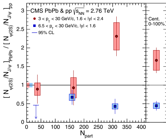
Fig. 93 Mid-rapidity (blue squares) and forward-rapidity (red circles, slightly shifted) double ratio of measured yields, (N_{\psi(2S)}/N_{J/\psi})_{PbPb} , as a function of centrality [686]. The centrality-integrated results are displayed in the right panel. Statistical (systematic) uncertainties are shown as bars (boxes). The boxes at unity indicate the (global) pp uncertainties
