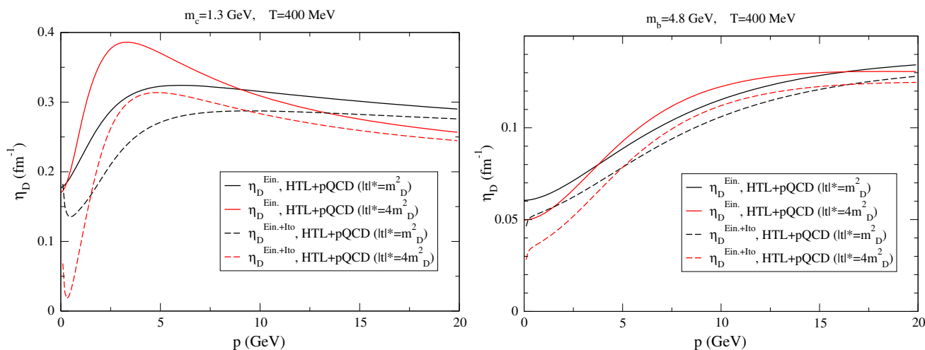
Fig. 60 The charm (left panel) and beauty (right panel) friction coefficients in a Quark Gluon Plasma at a temperature T = 400 MeV. Continuous curves refer to the results of the Einstein relation \eta_D = \kappa_L/2ET , while dashed curves include the discretisation correction in Eq. (31)
