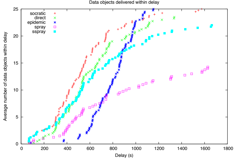
Figure 9: Average delay distribution in the disconnected scenario for the different representative replication approaches.
