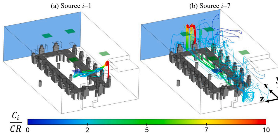
Fig. 7. Streamlines of the contaminant dispersion path from source location (a) i = 1 and (b) i = 7 , colored by the local concentration of that source, C_i , normalized by the room average breath-zone concentration from all the sources in this case, CR , referred to as the local case-normalized exposure from that source, C_i/CR . (For interpretation of the references to color in this figure legend, the reader is referred to the web version of this article.)
