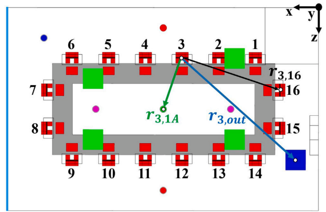
Fig. 2. Examples of the radius measures used to discuss the location based trends including the distance from Source 3 to the receiving Occupant 16, r_{3,16} (black), the distance from Source 3 to the room outlet, r_{3,out} (blue), and the distance from the Source 3 to the PAC 1 A, r_{3,1A} (green). (For interpretation of the references to color in this figure legend, the reader is referred to the web version of this article.)
