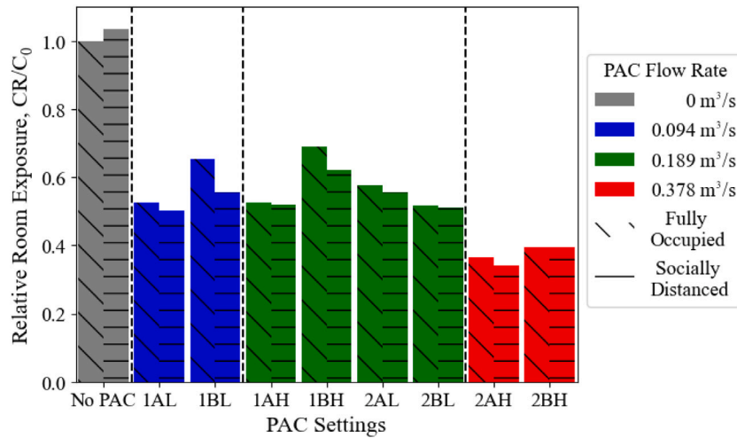
Fig. 13. Histogram of the room average breath-zone concentrations in each case, CR , normalized by the baseline concentration, C_0 .
