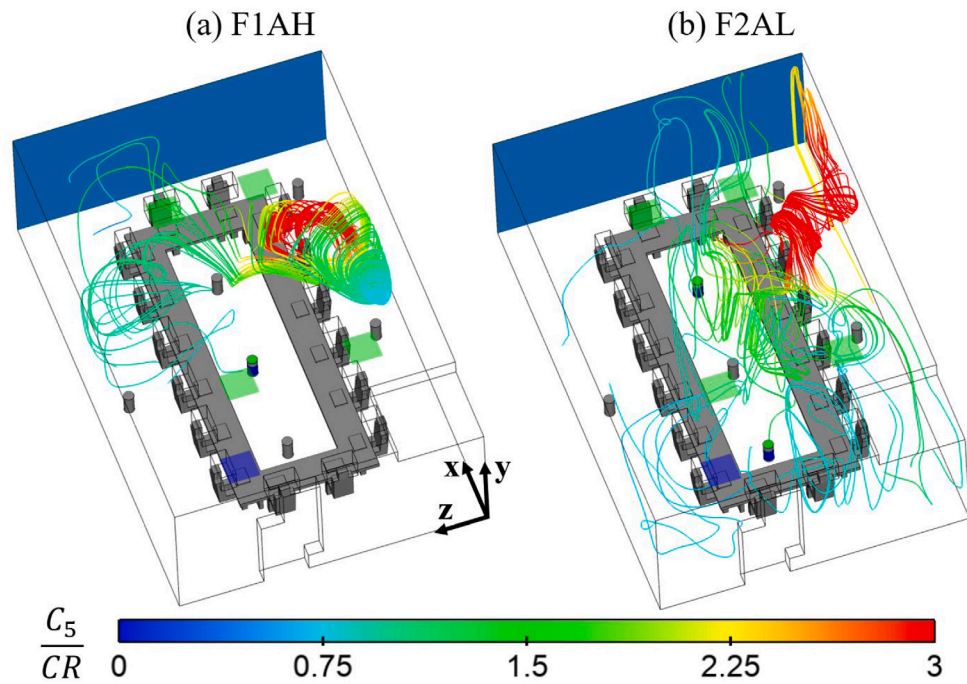
Fig. 15. This figure shows streamlines of the dispersion path of the contaminant from Occupant 5 colored by the local concentration of contaminant-5, C_5 , normalized by the room average breath-zone exposure, CR , for (a) case F1AH when the room is bifurcated along the x -axis direction, and (b) case F2AL when the room is bifurcated along the z -axis. (For interpretation of the references to color in this figure legend, the reader is referred to the web version of this article.)
