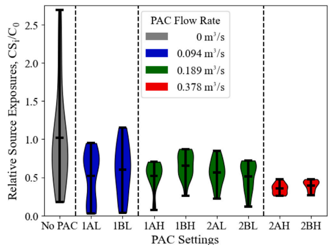
Fig. 10. Each violin-plot depicts the distribution of the source exposures, CS_i , relative to the baseline concentration, C_0 , at each PAC Setting, with the black lines representing the minimum, mean, and maximum values of each set, and the width representing the distribution of 16 source exposure (8 in each setup) within that range.
