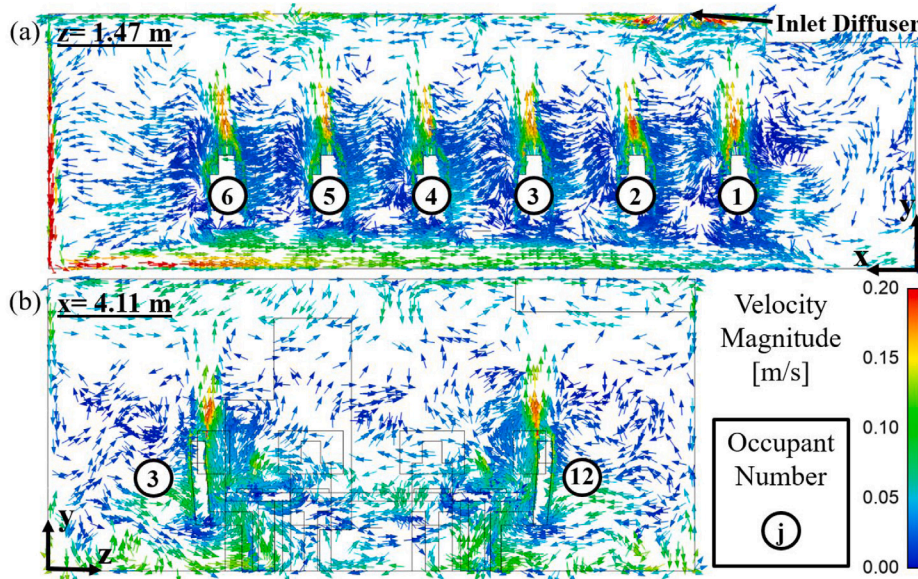
Fig. 4. Velocity field in the baseline case, F0, showing (a) a plane intersecting Occupants 1–6, 0.01 m from the occupants mouth plane, and (b) the plane bisecting Occupants 3–12.
