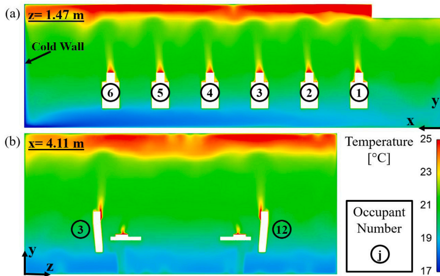
Fig. 3. Contours of temperature in the baseline case, F0, showing (a) a plane intersecting Occupants 1–6, 0.01 m from the occupants mouth plane, and (b) the plane bisecting Occupants 3–12.
