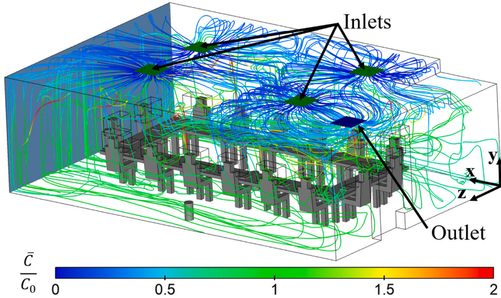
Fig. 5. Streamlines starting from the four ceiling inlet diffusers and colored by the average relative concentration, \bar{C}/C_0 . (For interpretation of the references to color in this figure legend, the reader is referred to the web version of this article.)
