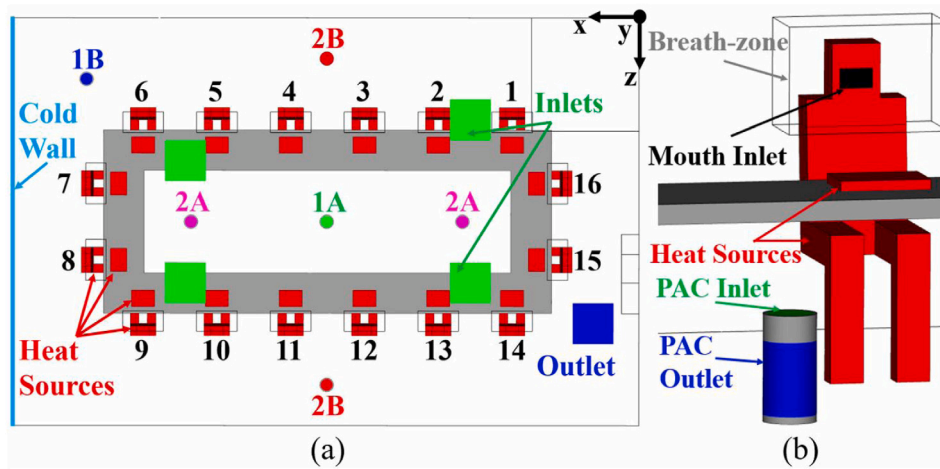
Fig. 1. Diagram of the domain boundary conditions including; (a) an overhead view of the fully-occupied room showing the positions of the ceiling inlets and outlet, the different PAC configurations, the cold external wall, and the occupants (numbered 1–16), while (b) shows a close up of one simulated occupants including their breath-zone, and the cylindrical PAC model used in this study. Note that ‘dirty’ air enters the PAC through the outlet surface (blue) and 100% clean air, c_i = 0 , enters the room through the inlet surface (green). (For interpretation of the references to color in this figure legend, the reader is referred to the web version of this article.)
