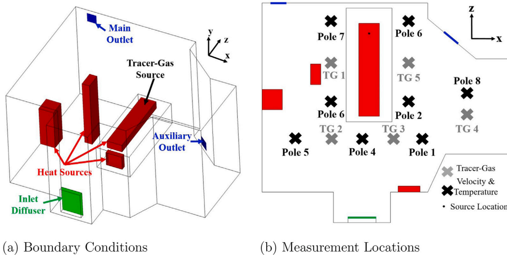
Fig. 17. Description of Yin et al. [33] experimental geometry and measuring locations used to validate the tracer-gas CFD model including (a) the major boundary conditions, and (b) the locations where vertical profiles of the tracer-gas concentration (gray) as well as temperature and velocity (black) were measured at six to eight points spaced vertically in the room. (For interpretation of the references to color in this figure legend, the reader is referred to the web version of this article.)
