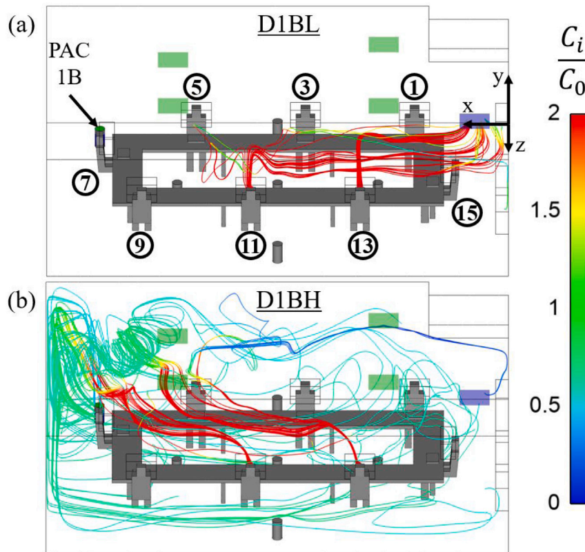
Fig. 9. Streamlines of the dispersion path from sources i = 11 and 13 for cases (a) D1BL, and (b) D1BH. In each case the streamlines are colored by the respective source-exposures, C_i , normalized by the reference concentration, C_0 . (For interpretation of the references to color in this figure legend, the reader is referred to the web version of this article.)
