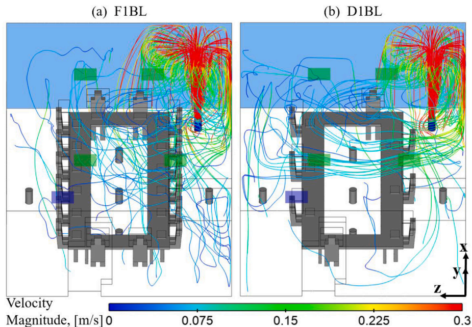
Fig. 16. Comparison of the streamlines, colored by the local velocity magnitude, coming from the PAC inlet in (a) the fully occupied and (b) the socially distanced room setups for the PAC setting 1BL. (For interpretation of the references to color in this figure legend, the reader is referred to the web version of this article.)
