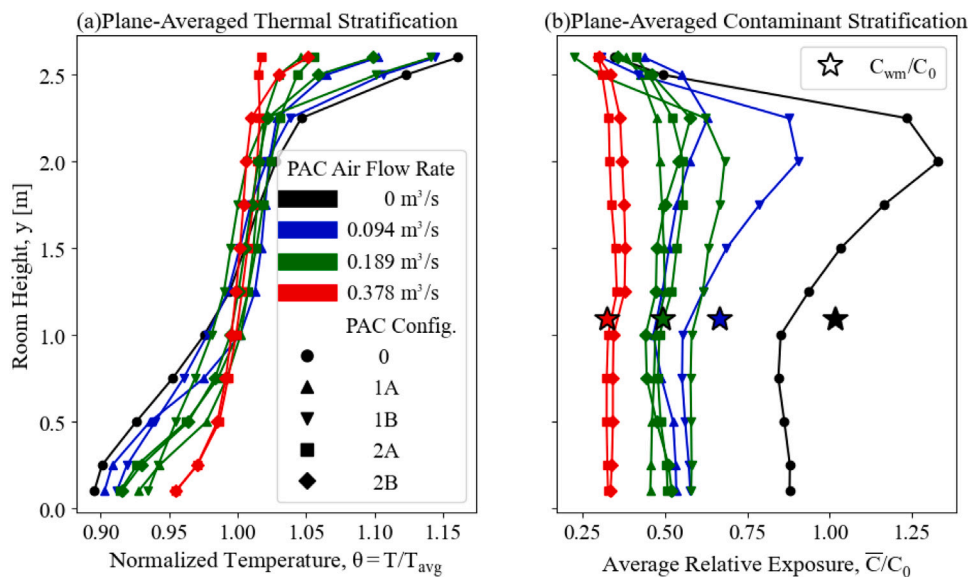
Fig. 8. Comparison of the (a) thermal and (b) contaminant stratification across the different PAC settings in the fully-occupied room set-up. The plots show the area-weighted average of their respective quantities for x-z cross-sections of the entire room-domain at the specified height in the room, y. (b) also shows the well-mixed relative exposure, C_{wm}/C_0 , for each flow rate, plotted (★) at the midpoint of the measured breath-zone ( y = 1.09 m) for ease of comparison to the exposure measures used in this study. (For interpretation of the references to color in this figure legend, the reader is referred to the web version of this article.)
