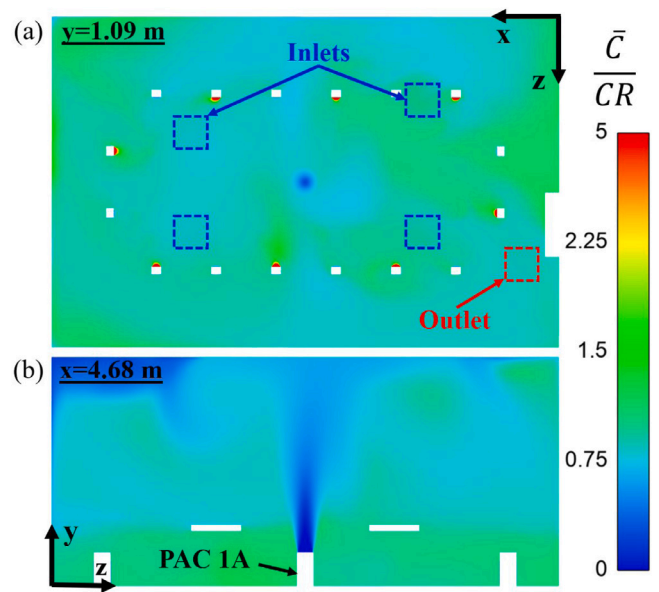
Fig. 14. Contours of the average contaminant concentration from all eight sources, \bar{C} , normalized by the room average breath-zone exposure, CR , for case F1AL shown at (a) the occupants breath-plane at the center of each mouth inlet, and (b) the mid-plane of the room bisecting PACs 1 A and 2B.
