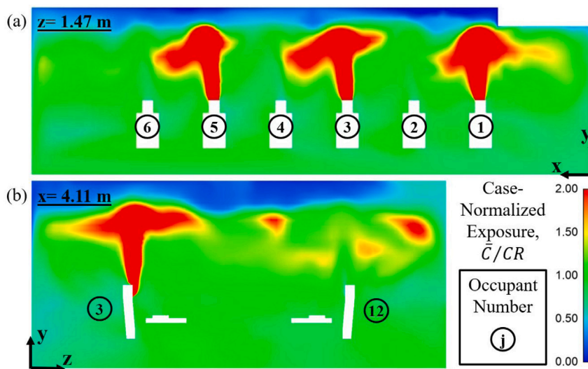
Fig. 6. Contours of the room averaged contaminant concentration, \bar{C} , normalized by the average breath-zone concentration in the baseline case, F0, showing (a) a plane intersecting Occupants 1–6, 0.01 m from the occupants mouth plane, and (b) the plane bisecting Occupants 3–12.
