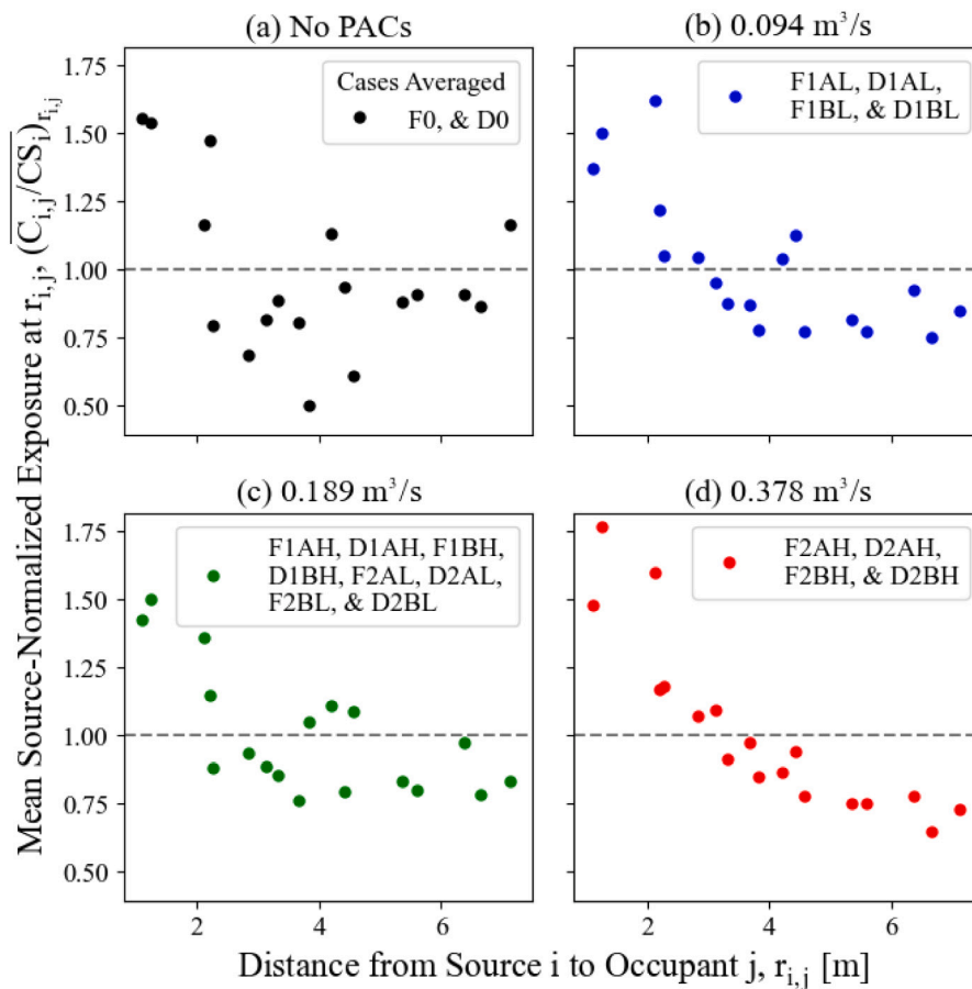
Fig. 12. The individual exposures, C_{i,j} , which have the same distance from the source to the receiving occupant, r_{i,j} , each normalized by the average exposure from the corresponding source, CS_i , averaged over all the cases at a particular PAC flow rate: (a) 0 \text{ m}^3/\text{s} , (b) 0.094 \text{ m}^3/\text{s} , (c) 0.189 \text{ m}^3/\text{s} , and (d) 0.378 \text{ m}^3/\text{s} . (C_{i,j}/CS_i)_{r_{i,j}} > 1 indicates a higher-than-average exposure at the distance r_{i,j} from the source- i across all cases at that flow rate.
