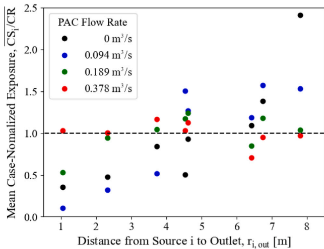
Fig. 11. This plot shows the source exposure, CS_i , normalized by the room average exposure for that case, CR . Averaged value at each location i is plotted against the sources distance from the room outlet over all the cases at the same PAC flow rate; 0 \text{ m}^3/\text{s} (black), 0.094 \text{ m}^3/\text{s} (blue), 0.189 \text{ m}^3/\text{s} (green), and 0.378 \text{ m}^3/\text{s} (red). (For interpretation of the references to color in this figure legend, the reader is referred to the web version of this article.)
