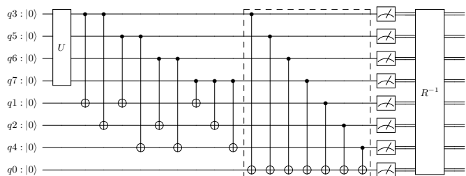
FIG. 4. Illustration of the encoding for the Hamming (8,4) code. The first four qubits (indexed q3, q5, q6, q7) contain logical state information while the remaining qubits are the parity bits. For the Hamming (7,4) code we omit the last parity bit (q0) and all gates connected to it, i.e. those within the black dashed box.
