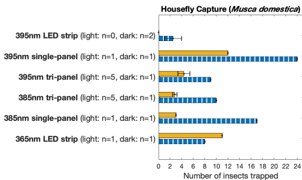
Fig. 8: Number of houseflies trapped (out of 50) after 2 hrs in cage with ICM affixed with LED cores of different wavelengths in regular (solid bars) and low (hatched bars) ambient lighting conditions, respectively. Parameter n refers to the number of trials, 50 flies/trial.
