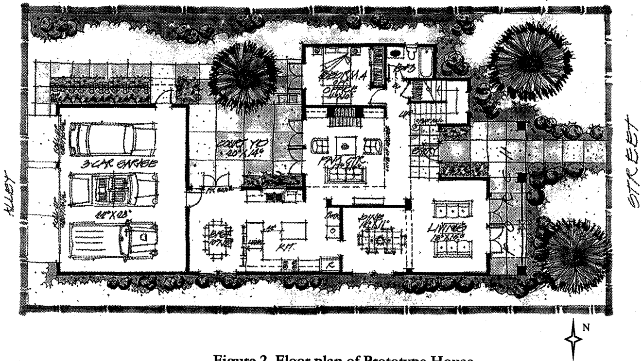
Figure 2. Floor plan of Prototype House
