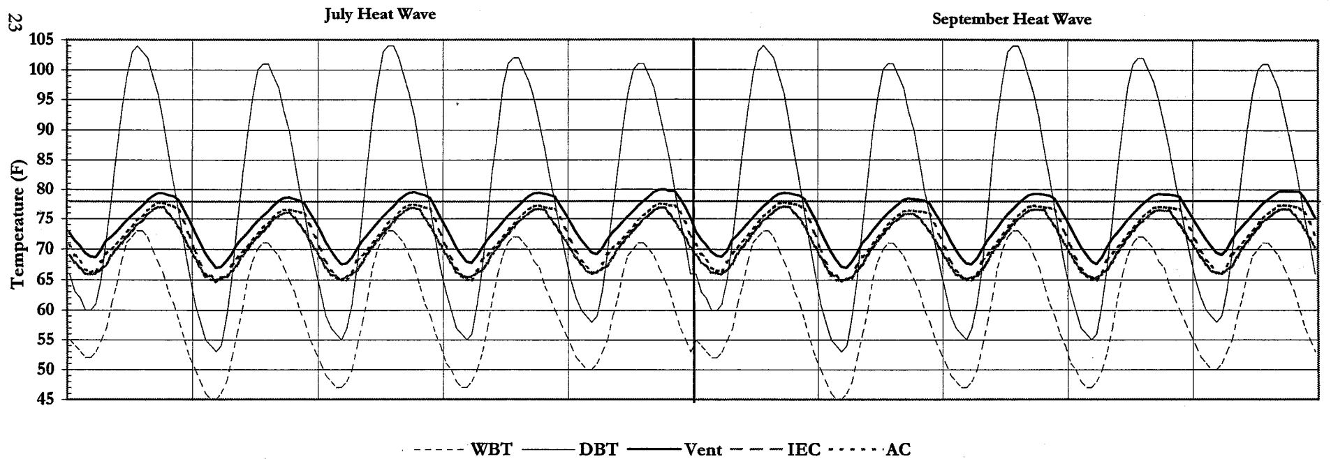
Figure 6. 1500 CFM system in Davis
