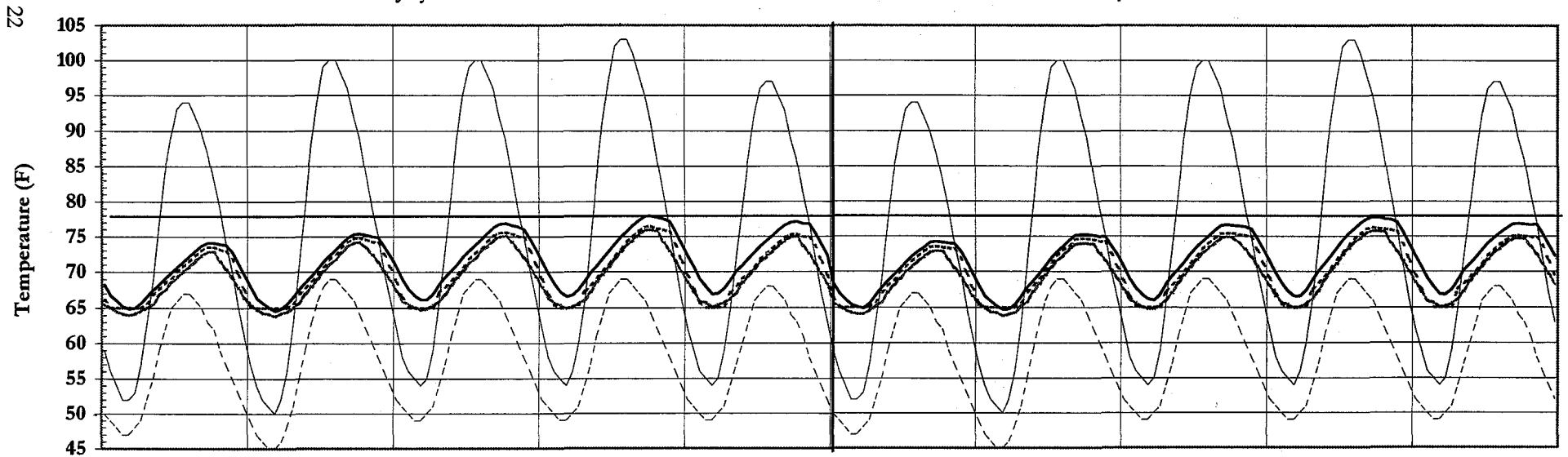
Figure 4. 1500 CFM system in Walnut Creek
