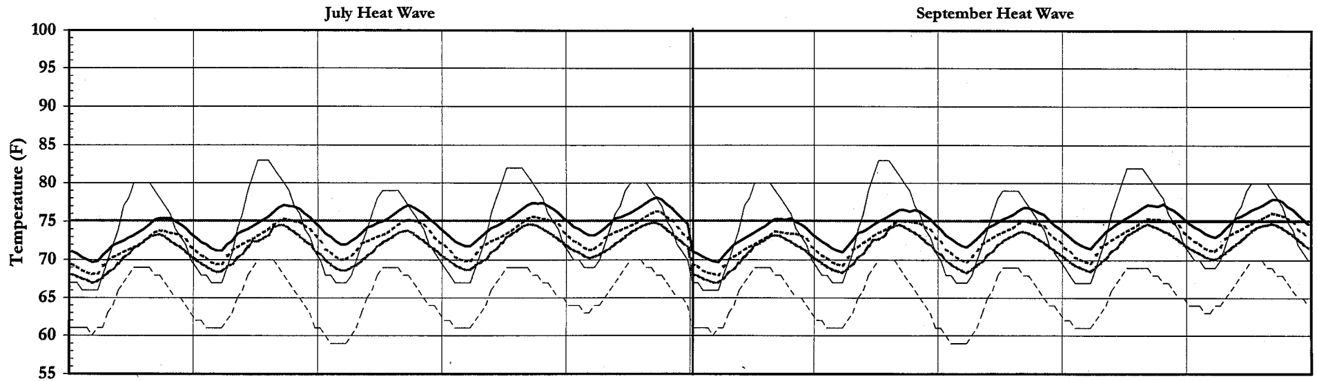
Figure 8. 1500 CFM system in Pasadena
