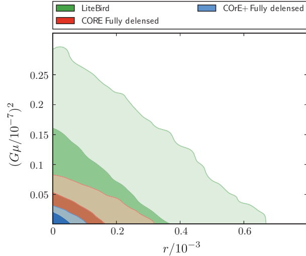
Figure 38: Likelihood contours of the r-(G\mu)^2 posterior for models with both tensors and defects (cosmic strings), marginalized over all other parameters, for LiteBIRD, CORE, and CORe+. The CORE and CORe+ contours are given for the fully delensed case, representing the best possible constraints attainable, while LiteBIRD contours are given for the standard case. In all cases light shading represents 1\sigma and dark shading 2\sigma . For comparison, the current Planck marginalized 95% confidence limits on these models are (G\mu/10^{-7})^2 < 3.4 ( f_{10} < 0.011 ) and r < 0.11 .
