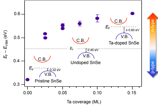
Figure 3: (Color online) The VBM ( E_{VBM} ) relative to E_F as a function of Ta coverage. While the energy gap is 0.9 eV (32; 33), the criterion determining the carrier type is considered to be 0.45 eV denoted by the dashed line. A pristine sample gives E_F - E_{VBM} = 0.32 eV, indicating p -type carriers. Ta adsorption leads to the shift of the VBM, indicating the change of charge carrier type to n -type.
