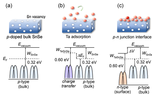
Figure 4: (Color online) (a-c) Upper panels show schematics of the formation of a p - n junction interface between p -doped SnSe bulk and Ta-adsorbed SnSe surface. Lower panels show the change of an energy band diagram upon Ta adsorption.
