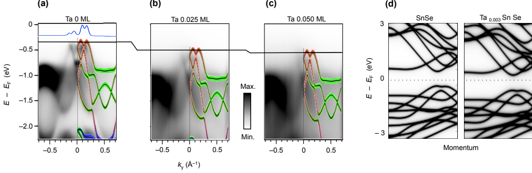
Figure 2: (Color online) (a-c) ARPES intensity maps of SnSe taken along \Gamma - Y direction for three different Ta coverages, 0 ML, 0.025 ML, and 0.050 ML. The blue curve is a momentum distribution curve taken at the valence band maximum, i. e., 0.32 eV below E_F . The calculated electron band structure of SnSe by the TB-mBJ method is rigidly shifted to fit to the ARPES data. Red, green, and blue color in the calculated band denotes Se p_x , p_y , and p_z orbitals, respectively. The black line denotes the shift of the valence band maximum. (d) The calculated electron band structure of SnSe with and without Ta by the KKR green function method.
