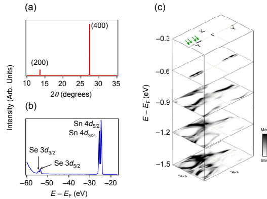
Figure 1: (Color online) (a) X-ray diffraction data for single crystal SnSe with Sn-vacancy. (b) X-ray photoemission spectrum for single crystal SnSe with Sn-vacancy. (c) Constant energy maps taken using ARPES at E - E_F = -0.3, -0.6, -0.9, -1.2, and -1.5 eV.
