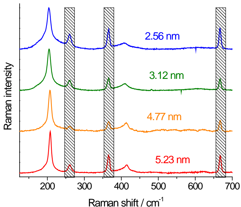
Figure 2. Resonance Raman spectra excited near the lowest excitonic absorption maximum. Excitation wavelengths are, from top to bottom, 514.5 nm, 532 nm, 594 nm, and 594 nm. Shaded bars mark chloroform solvent lines whose intensity relative to that of the CdSe NCs varies with both Raman cross-section and sample concentration. The spectra are parallel polarization only for the 594 nm excited samples, and parallel plus perpendicular for the other two.
