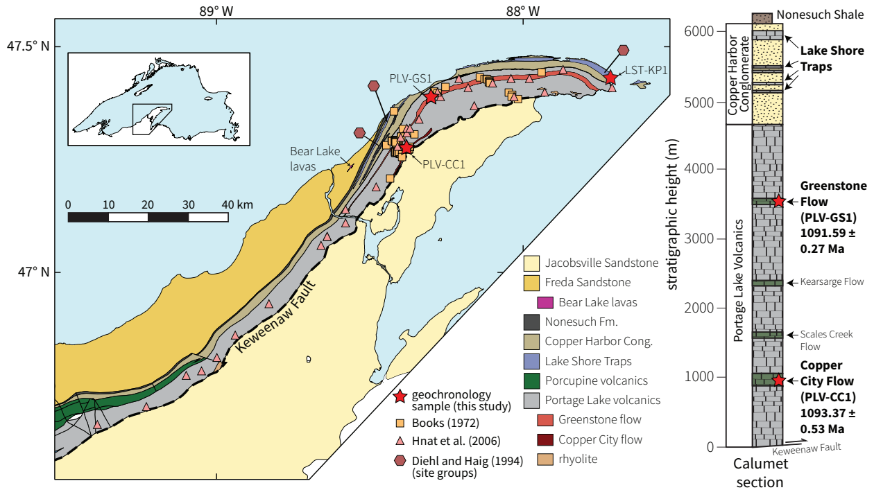
Figure 7. Geological map of the Keweenaw Peninsula, northern Michigan, and summary stratigraphy of the Portage Lake Volcanics and Copper Harbor conglomerate from a section near Calumet both modified from Cannon and Nicholson (2001). The position of paleomagnetic sites from Books (1972) and Hnat et al. (2006) used for the Portage Lake Volcanics pole and the localities of Diehl and Haig (1994) site groupings within the Lake Shore Traps are shown. The U-Pb dates shown for the Copper City Flow and the Greenstone Flow are from this study.
