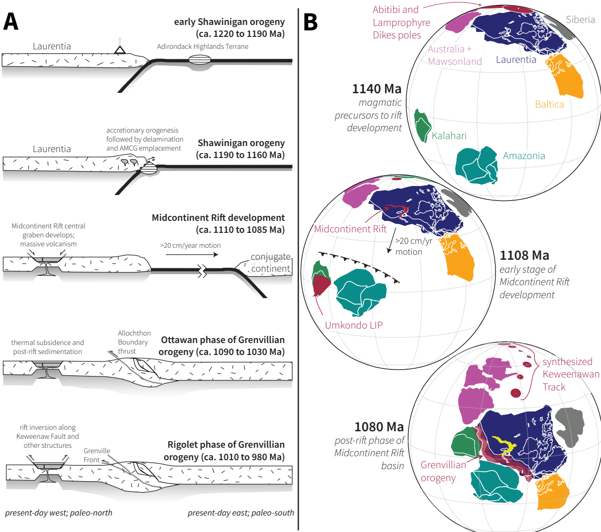
Figure 12. A: Schematic cartoons of the development of the Midcontinent Rift in the context of Grenville margin orogenesis. The schematic transect extends from the interior of the Laurentia where the Midcontinent Rift developed to the margin of Laurentia in the vicinity of the modern day Adirondacks. The timescale and geometry of the Shawinigan orogeny follows that of McLelland et al. (2013), while the timing and geometry of the Allochthon Boundary thrust and the Grenville Front follows that of Hynes and Rivers (2010). These cross-sections are schematic and not to scale. B: Paleogeographic reconstructions on an orthographic projection before, during and after active extension within the Midcontinent Rift. The positions of Baltica and Amazonia relative to Laurentia follows Evans (2013) with slight modifications. The ca. 1140 Ma reconstruction is consistent with the ca. 1150 Ma Fortuna Formation pole for Amazonia (D’Agrella-Filho et al., 2008) and the ca. 1140 Ma Abitibi and lamprophyre dike poles of Laurentia (Ernst and Buchan, 1993; Piispa et al., 2018). The position of Kalahari relative to Laurentia follows Swanson-Hysell et al. (2015), Australia relative to Laurentia follows Swanson-Hysell et al. (2012) and Siberia relative to Laurentia follows Ernst et al. (2016) and Evans et al. (2016).
