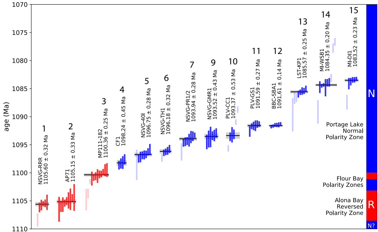
Figure 2. Date distribution plots for CA-ID-TIMS ^{206}\text{Pb}/^{238}\text{U} dates from the Midcontinent Rift colored by magnetic polarity (red for reversed, blue for normal). Vertical bars represent 2\sigma analytical uncertainty of individual zircon analyses; darker bars are data used in age calculations while light bars were excluded based on interpreted inheritance or Pb-loss. Horizontal lines and shaded bands signify weighted mean dates and their 2\sigma uncertainties. All dates are from this study with the exception of MP111-182 which was published in Swanson-Hysell et al. (2014a) and BBC-SBA1/MI-WSB1/MI-DI1 which were published in Fairchild et al. (2017). See Table S1 in Data Repository Item for complete U-Pb data, as well as the text and Table 1 for details regarding the geochronology. The interpreted geomagnetic polarity timescale is shown to the right. The geomagnetic reversal associated with the end of the Alona Bay reversed-polarity zone and the normal to reversed reversal within the Flour Bay polarity zones are constrained to have occurred between 1105.15 \pm 0.33 Ma and 1100.36 \pm 0.25 Ma. The geomagnetic reversal associated with the start of the Portage Lake normal-polarity zone is constrained to have occurred between 1100.36 \pm 0.25 Ma and 1098.24 \pm 0.45 Ma.
