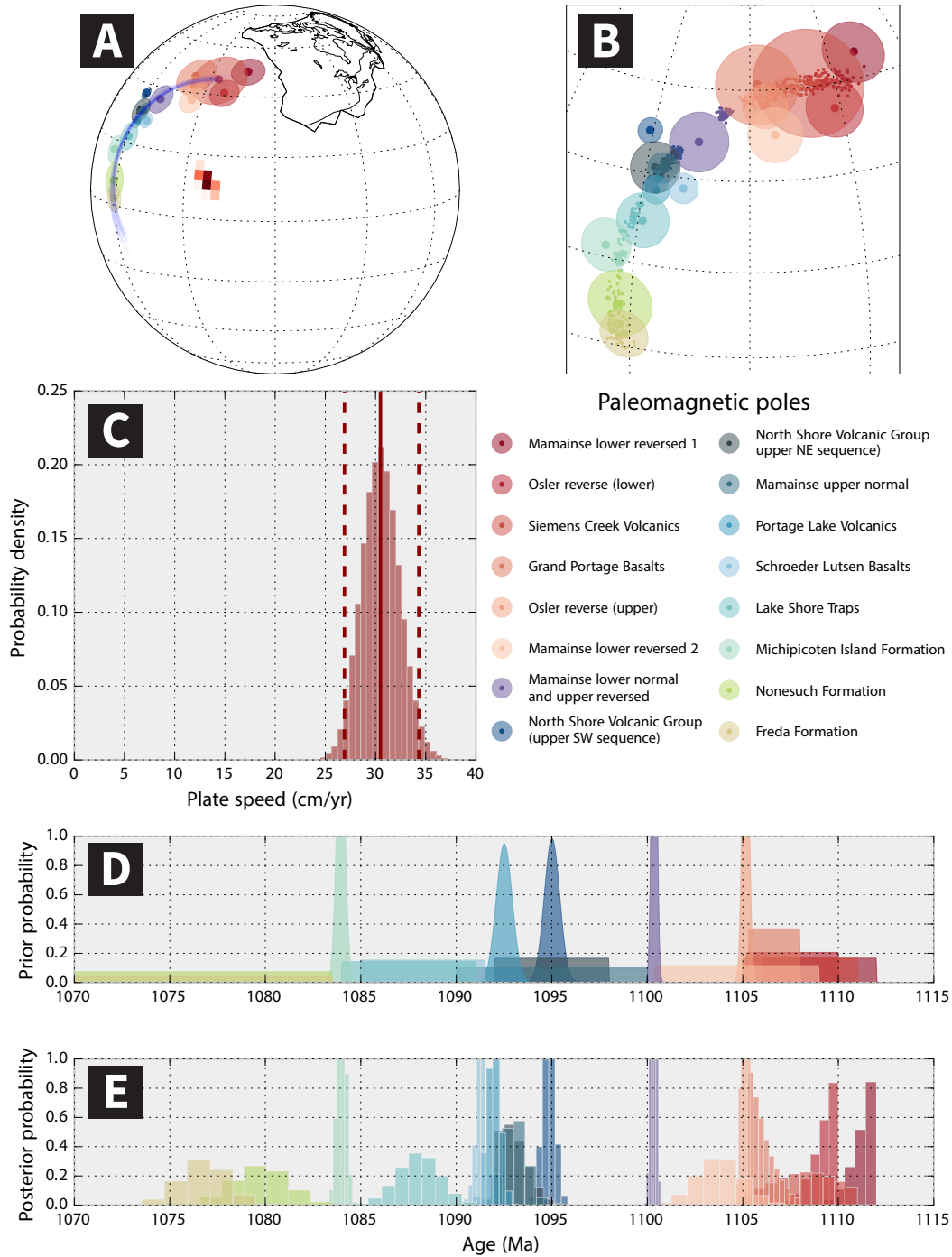
Figure 10. Inversion of the Keweenaw track for a single Euler rotation using the Bayesian framework discussed in the text. A: Euler pole locations developed through the inversion shown as a density plot along with a representative resulting tracks drawn over the paleomagnetic poles. B: Paleomagnetic pole positions for draws from the posterior distribution of the inversion superimposed on observed pole positions and their uncertainty. C: Laurentia plate speed distribution from the inversions. The solid line shows the median plate speed (31 cm/yr) and the dashed lines show the 95% credible interval (27-34 cm/yr). D: Prior probability distributions for the ages of the paleomagnetic poles. Poles with radiometric ages are given Gaussian prior distributions. Poles with stratigraphic age control are given uniform prior distributions between bracketing ages. E: Posterior probability distributions for the ages of the poles resulting from the inversion.
