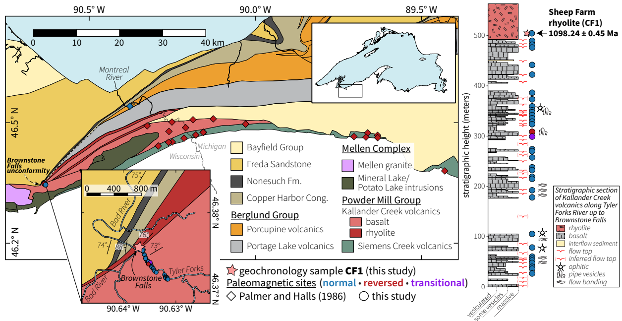
Figure 8. Geological map modified from Cannon et al. (1996) focused on the Powder Mill Group in northern Wisconsin and the westernmost part of Michigan’s upper Peninsula. The position of paleomagnetic sites deemed to have primary remanence from Palmer and Halls (1986) and those from this study are shown. The zoom-in map is centered Brownstone Falls within Copper Falls State Park and shows the location of the upper Kallander Creek Volcanics sites of this study and the Sheep Bed rhyolite geochronology sample. The stratigraphic column is of the upper 560 meters of the Kallander Creek Volcanics measured where the volcanics were sampled along the Tyler Forks River.
