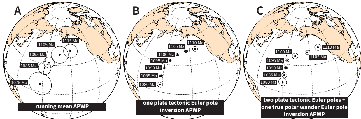
Figure 9. Synthesized stage poles associated with apparent polar wander paths for the Keweenaw Track. A: Running mean poles. B: 1 Euler pole inversion. C: 2 plate tectonic Euler pole + 1 true polar wander Euler pole inversion.
