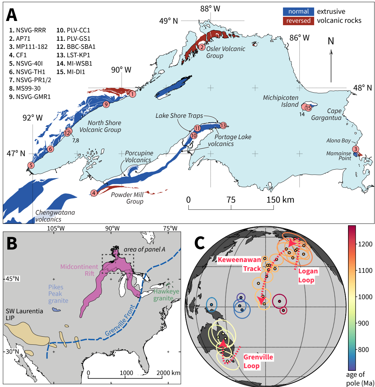
Figure 1. A: Geological map of Midcontinent Rift volcanics in the Lake Superior Region. The geomagnetic polarity is indicated by red (reversed) and blue (normal). Volcanic successions referred to in the text are labeled and the locations of geochronology samples are shown with circles and numbers that are keyed out to the sample name. B: Map of North America showing the position of the Midcontinent Rift inferred from surface geology and gravity anomaly data along with other ca. 1.1 Ga volcanic rocks including the SW Laurentia large igneous province (from Bright et al., 2014) and the Hawkeye Granite (from McLelland et al., 2010) as well as the the Grenville Front (from Rivers, 2015) . C: Overview of Laurentia’s apparent polar wander path from 1300 Ma to 700 Ma with the oldest pole coming from the Mackenzie large igneous province (ca. 1267 Ma) and the youngest from the Franklin large igneous province (ca. 720 Ma). The poles progress through the Logan Loop, the Keweenaw Track and the Grenville Loop.
