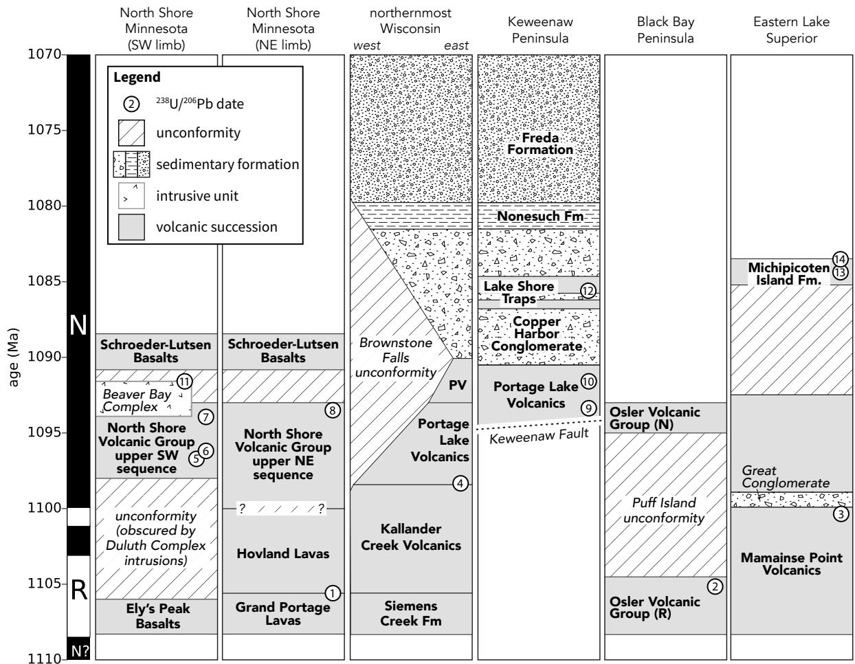
Figure 3. Chronostratigraphic correlation of Midcontinent Rift volcanic sequences informed by new U-Pb dates. The numbered circles correspond to CA-ID-TIMS ^{206}\text{Pb}/^{238}\text{U} dates using the same numbering scheme as in Figures 1 and 2. The analytical uncertainty, which should be used when comparing these dates to one another, is less than the time represented by the height of the circles. Extrapolated eruption rates, paleomagnetic data (both polarity and pole position) and ^{207}\text{Pb}/^{206}\text{Pb} dates (not shown) inform the chronostratigraphic interpretation, but the chronostratigraphy is most robust in the proximity of the ^{206}\text{Pb}/^{238}\text{U} dates. PV: Porcupine Volcanics; Fm: Formation.
