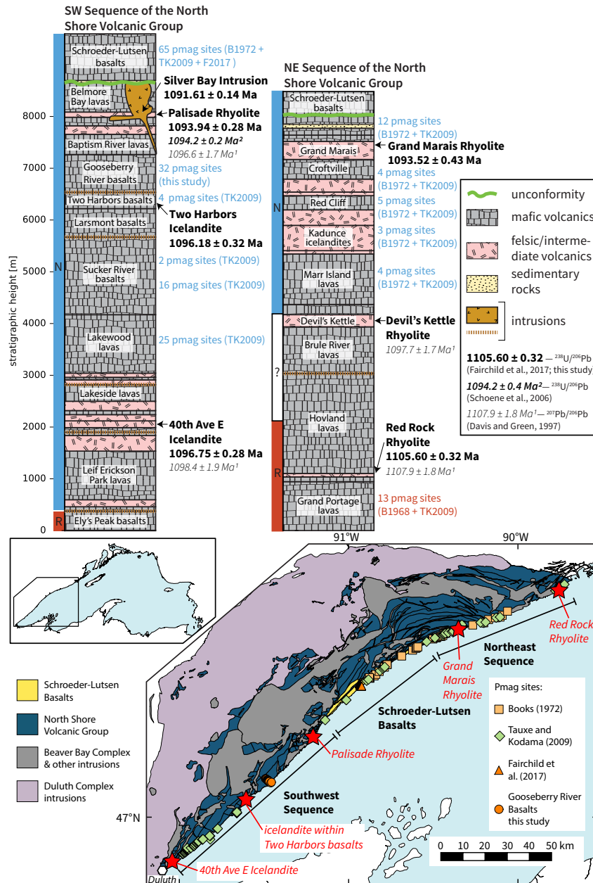
Figure 6. Geological map and summary stratigraphy of the North Shore Volcanic Group and Schroeder-Lutsen Basalts in northern Minnesota. Geologic map data are simplified from Miller et al. (2001). Stratigraphic columns are divided into the lithostratigraphic units of Green (2002) and the position of paleomagnetic sites and U-Pb dates are shown. Codes for the references associated with paleomagnetic sites are: B1968: Books (1968), B1972: Books (1972), TK2009: Tauxe and Kodama (2009), F2017: Fairchild et al. (2017). U-Pb dates are keyed out to indicate the reference and whether they are 206 Pb/ 238 U or 207 Pb/ 206 Pb dates. Dates from this study and Fairchild et al. (2017) are the most directly comparable and are used for constraining the age of paleomagnetic poles. The reversed geomagnetic polarity shown for the Ely's Peak basalts and the lower half of the Hovland lavas is from unpublished data developed by Ken Books at the USGS that has been reported in Minnesota Geological Survey maps.
