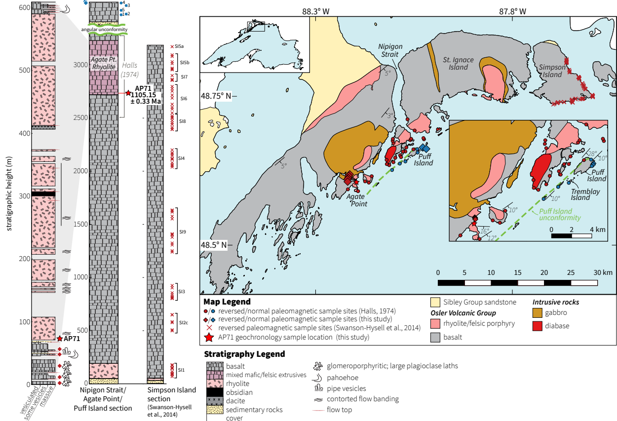
Figure 4. Geological map and summary Midcontinent Rift stratigraphy of the Lake Superior Archipelago, Ontario, Canada. Composite stratigraphic columns with the position of paleomagnetic sites from Halls (1974), Swanson-Hysell et al. (2014b) and this study are shown for the Nipigon Strait/Agate Point/Puff Island region and for Simpson Island. The Halls (1974) sites are in the upper portion of the stratigraphy as indicated with the red bracket. Exposures of extrusive rhyolitic lava flows occur on Agate Point with basaltic lavas below and above. The more detailed stratigraphic section for Agate Point shows the position of the dated rhyolite (AP71). The geological map is modified from Carter et al. (1973). The map, and the zoomed-in inset, show the position of the Puff Island unconformity and sample sites.
