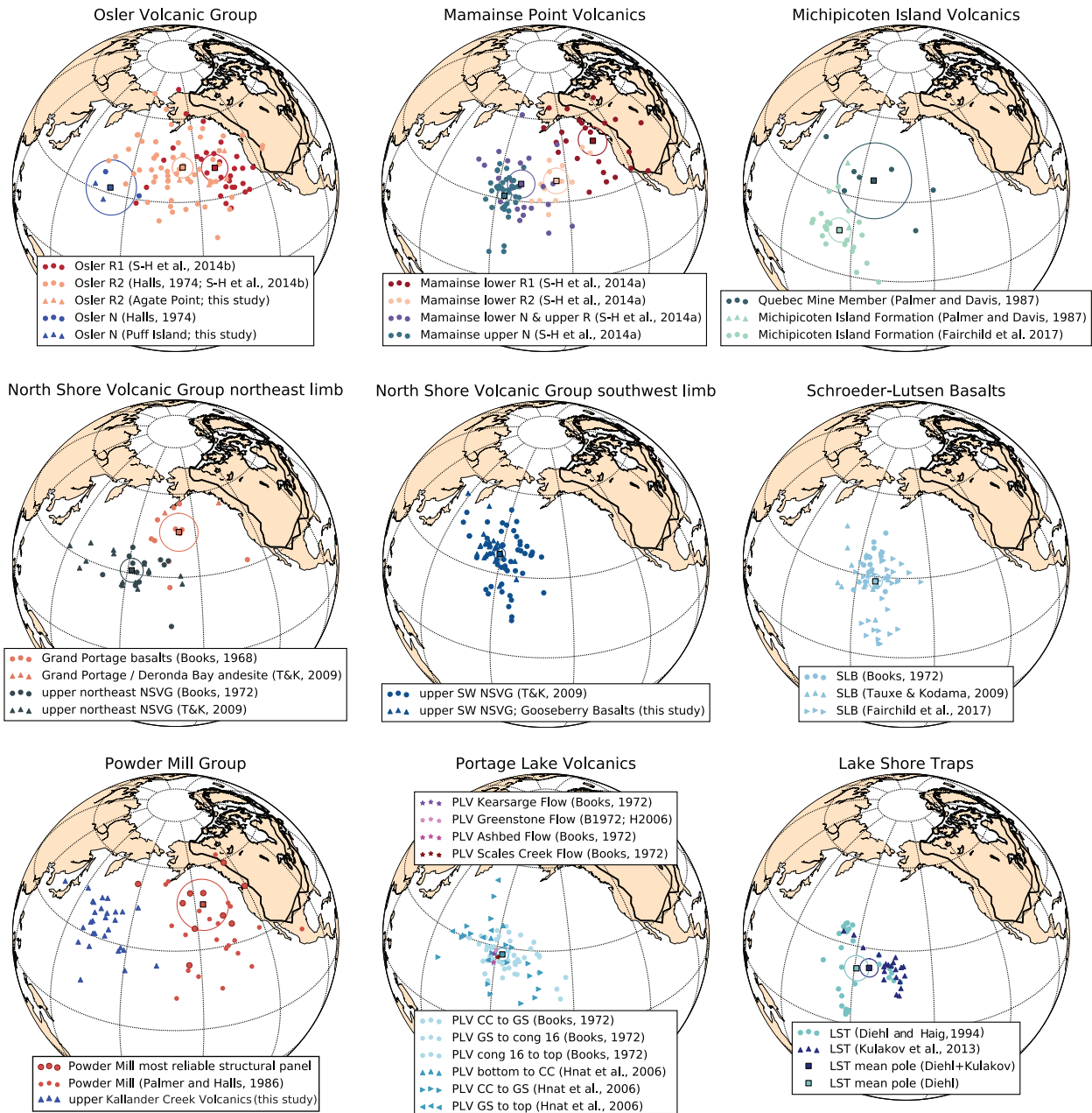
Figure 5. Virtual geomagnetic poles (VGPs) and mean paleomagnetic poles from extrusive volcanics of the Midcontinent Rift. VGPs from individual cooling units are shown as circles, triangles and stars color-coded to portions of the volcanic successions. Mean paleomagnetic poles calculated from these VGPs are shown as squares with associated A_{95} confidence ellipses. ‘T&K, 2009’ refers to Tauxe and Kodama (2009) and ‘S-H et al., 2014a’ and ‘S-H et al., 2014b’ refer to Swanson-Hysell et al. (2014a,b).
