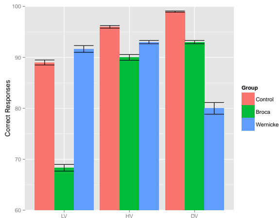
Figure 4: Percentage of correct responses by verb type and experimental group. Error bars indicate the standard error of the mean.
