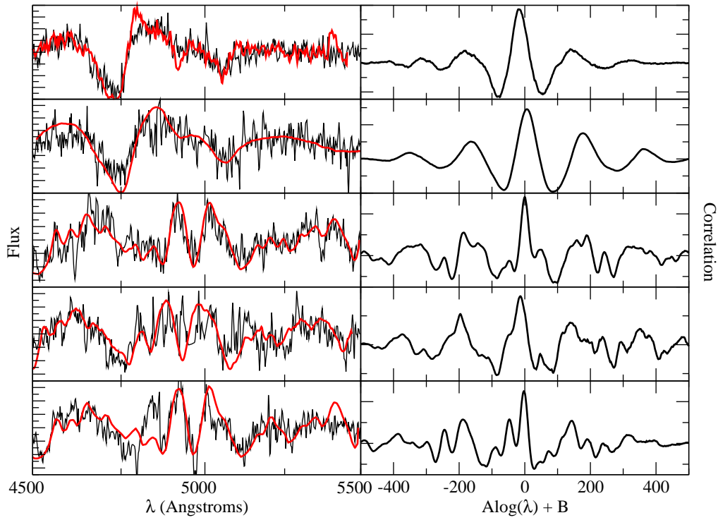
Fig. 12.— Left-hand-side : A plot of the best fit template spectrum (thick line) and the SNLS SNe II-P (thin line) used in the cross-correlation technique. Right-hand-side : The resultant correlation. Plotted from top to bottom are: SNLS-03D3ce, 03D4cw, 04D1ln, 04D1pj and 04D4fu.
