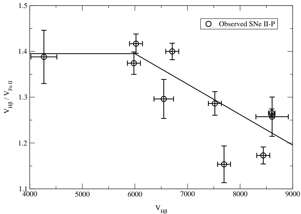
Fig. 3.— The ratio of the velocities of H\beta to Fe II 5169\text{\AA} vs. the H\beta velocity in the H\beta -dominated spectra. We fit this ratio in two pieces, a constant for velocities below 6000 km/s ( ratio = 1.395 ) and linearly for higher velocities ( ratio = 1.395 - 6.489 \times 10^{-5}(V(H\beta) - 6000) ). The linear portion is the only one relevant to our analysis as our high-redshift data lie within these velocities. The dispersion about this relationship ( \pm 0.054 ) translates to an uncertainty in measuring the Fe II velocity from H\beta of \sim 300 km/s. See text for a full discussion and explanation of this trend.
