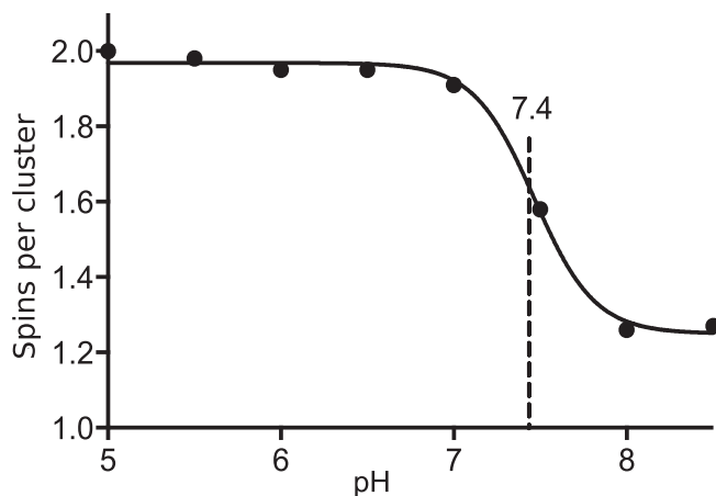
Fig. 3. mVDAC1 forms a dimer at low pH. Titration curve of mVDAC1 D100R1 at eight different pH values. All samples were measured at 100 \mu M, and the modulation depth was used to calculate the number of spins per cluster using Eq. 3. Data were fitted using PRISM software, revealing a sharp transition with a midpoint value of 7.4. The dipolar evolution functions and distance distributions are displayed in Fig. 55.
