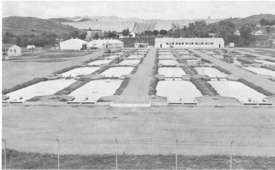
FIGURE 45. Standard California type earthfill rearing ponds, San Joaquin Hatchery. The ponds are 100 feet long and are arranged in series of 6 ponds. Each series requires 3\frac{1}{2} cfs of water. Friant Dam, which forms Millerton Lake, is in background. Photograph by William M. Carah, May 1956.
