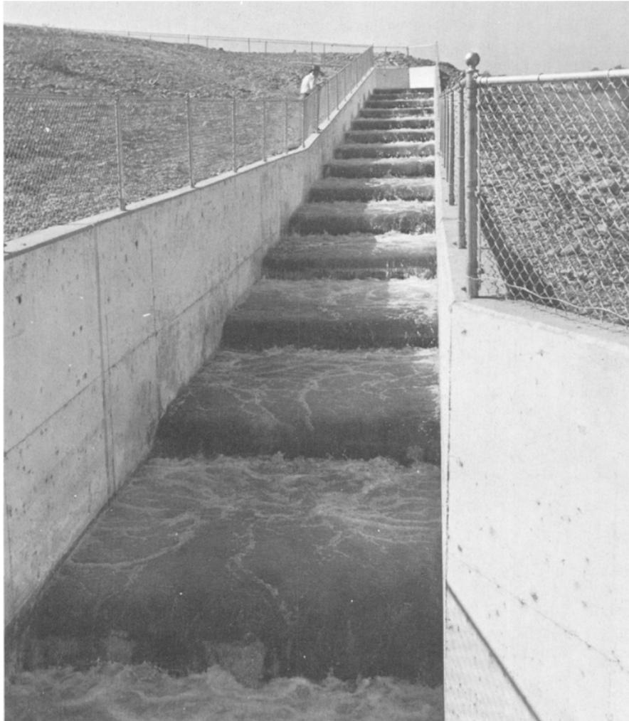
FIGURE 55. Fish ladder, Nimbus Hatchery. The pools are 12 feet long, 9 feet wide, and 8 feet deep. There is a 1-foot jump between pools. Adult salmon and steelhead negotiate this ladder with ease.
